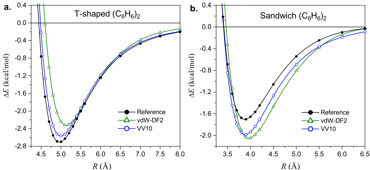
FIG. 3. Interaction energy curves for (a) the T-shaped and (b) the stacked sandwich-shaped benzene dimers. R is the distance between the centers of mass of the monomers. Reference values are from Ref. 32. VV10 and vdW-DF2 results were obtained self-consistently with the aug-cc-pVTZ basis set.
