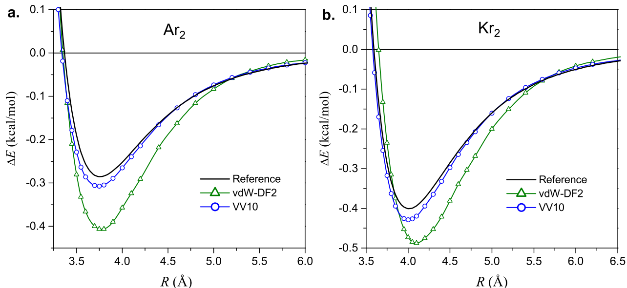
FIG. 1. Interaction energy curves for (a) the argon dimer and (b) the krypton dimer. Reference curves are from Ref. 31. VV10 and vdW-DF2 results were obtained self-consistently with the aug-cc-pVQZ basis set.
