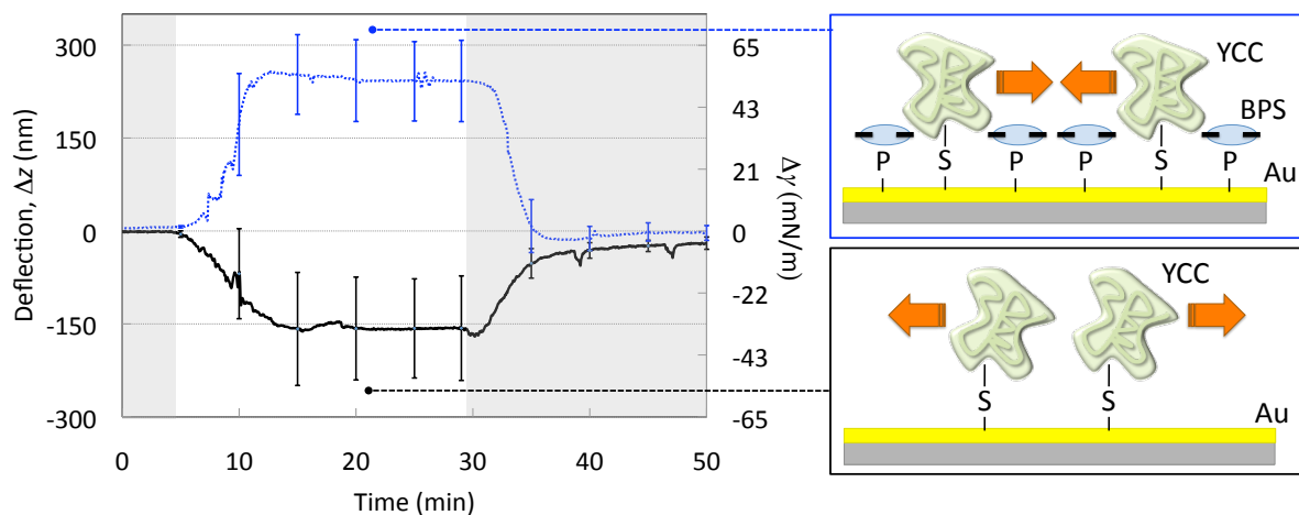
Figure 3. Left panel. Mean differential deflection signals (left ordinate axis) and mean differential surface pressure (right axis) of the YCC-Au MCs (black solid line) and of the YCC-BPS-Au MCs (blue dashed line) when the solution is cycled from 50 mM PBS (grey area) to 10 mM PBS (white area). Right top panel. Scheme of the top face of a YCC-BPS-Au MC and of the in-plane inter-protein attractive forces that are triggered by the salt concentration decrease and cumulate to deflect the MC upward. Right bottom panel. Scheme of the top face of a YCC-Au MC and of the in-plane inter-protein repulsive forces that are triggered by the salt concentration decrease and cumulate to deflect the MC downward.
