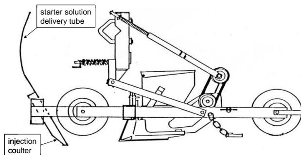
Fig. 2. Stanhay seed drill showing position of commercial prototype injection coultter.
