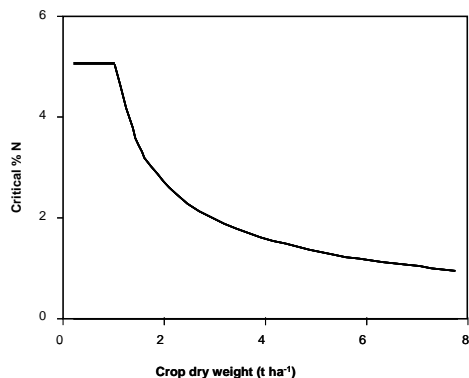
Fig. 1 Changes in plant critical N concentration during growth.
