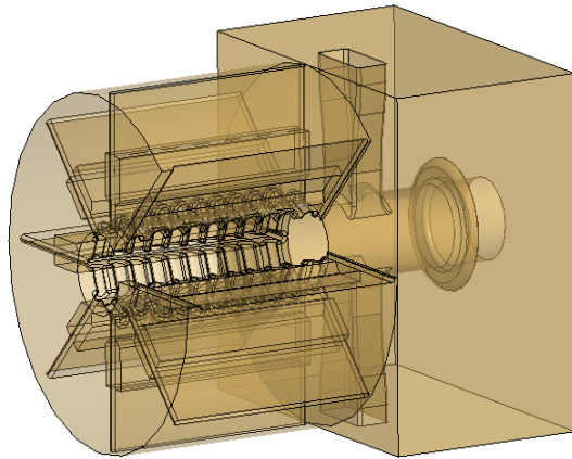
Figure 2: The CLIC PETS general view
