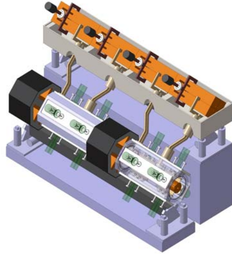
Figure 1: The CLIC module layout
