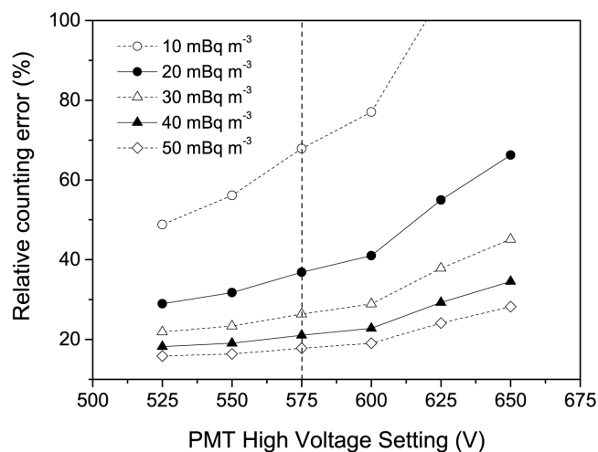
Figure 4. Relative counting error as a function of photomultiplier operating voltage for nominal radon concentrations between 10 and 50 \text{ mBq m}^{-3} . The KSG detector's current operating voltage is indicated with a vertical dashed line.
