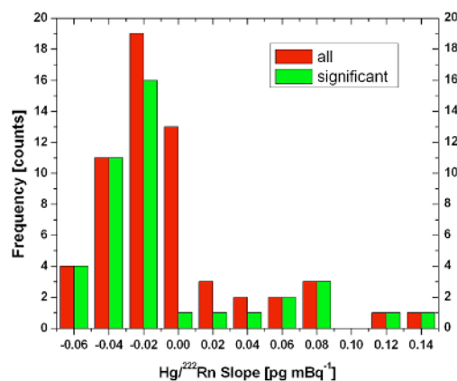
Fig. 1 Frequency distribution of GEM/Rn slopes.
