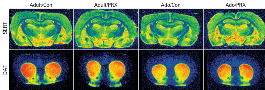
Fig. 6. Representative autoradiograms demonstrating [ ^{125}\text{I} ]RTI-55 binding to the serotonin transporter (SERT) and dopamine transporter (DAT). SERT binding density was measured in the CA3 region of the hippocampus and basolateral amygdala (Bregma -2.7 ), while DAT binding was measured in the medial and lateral caudate putamen and nucleus accumbens core (Bregma +1.3 ).
