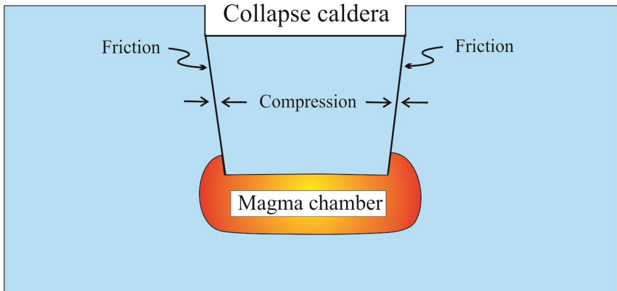
Fig. 7. Schematic illustration of caldera subsidence on an inward-dipping normal ring-fault. As the caldera block subsides, it becomes subject to higher horizontal compression (compressive stress). So long as no ring-dyke is injected along the fault, the friction together with the normal stress on the ring-fault ensure that the fault remains closed and the displacement stable. Thus, collapse on an inward-dipping normal ring-fault is less likely than an outward-dipping ring-fault to result in increasing volumetric flow rate (Eq. 1) through a ring-dyke as the subsidence increases. Also, the magma chamber is here unlikely to be destroyed during the collapse.
