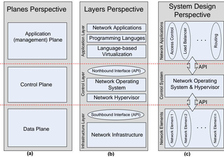
Figure 4. SDN perspectives in planes, layers and system design architecture (inspired by [34,39,40]) (a) Planes Perspective, (b) Layers Prescriptive, (c) System Design Perspective
