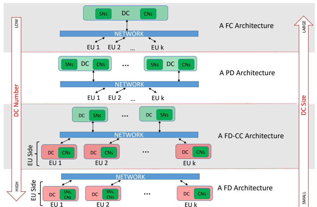
Figure 2. The Cloud architecture taxonomy; ranging from fully centralized to fully distributed [12].
