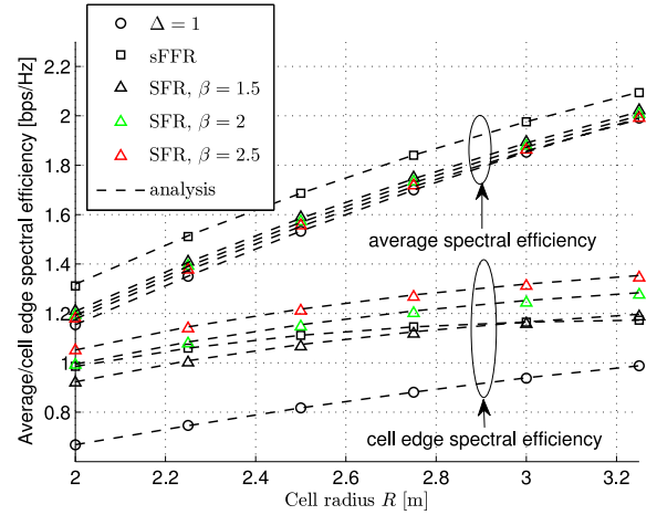
Fig. 11. Average spectral efficiency and cell edge spectral efficiency against cell radius R . System parameters: \delta = 0.7 , N_0 = 1 \times 10^{-21} \text{ A}^2/\text{Hz} and \lambda = 1 \text{ user}/\text{m}^2 .
