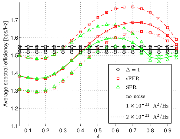
Fig. 12. Average spectral efficiency against \delta . System parameters: R = 2.5 \text{ m} , \lambda = 1 \text{ user}/\text{m}^2 and \beta = 2 .
