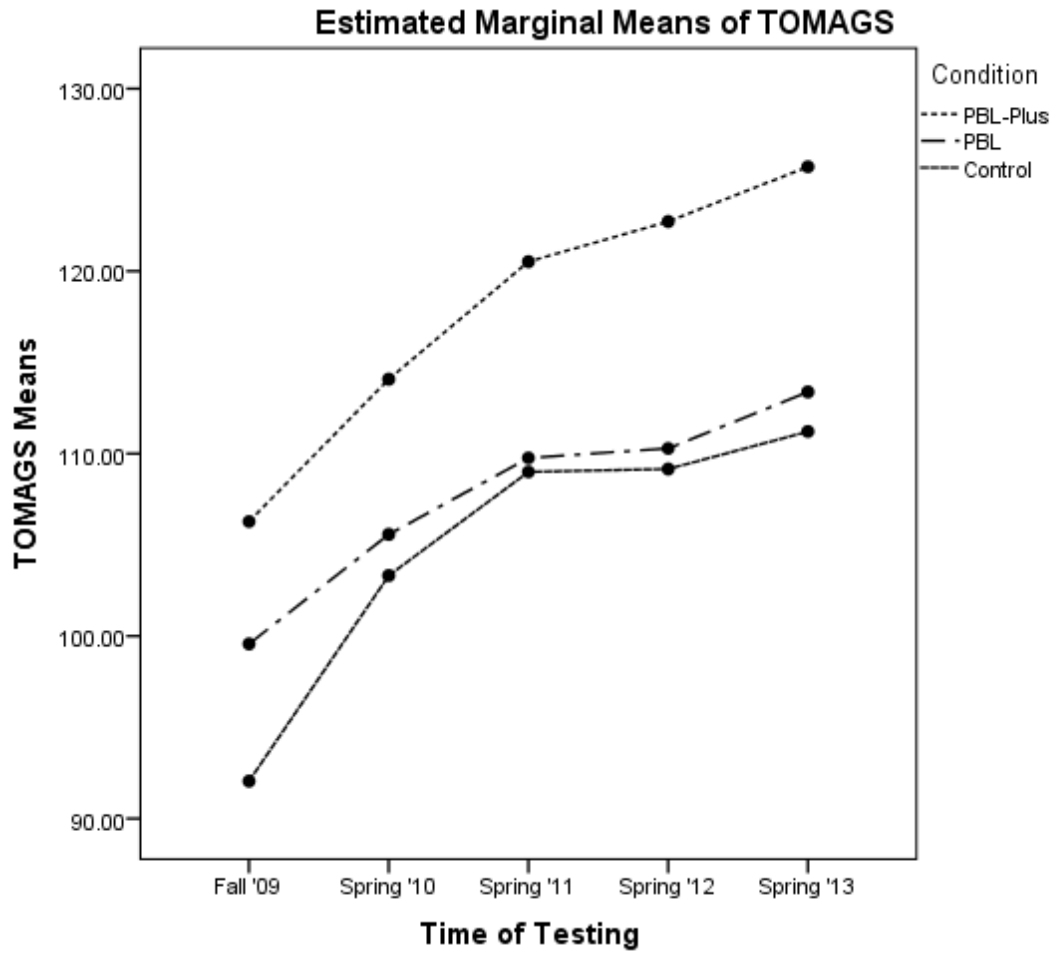
Figure 1. Estimated marginal means for TOMAGS scores by group across time.
