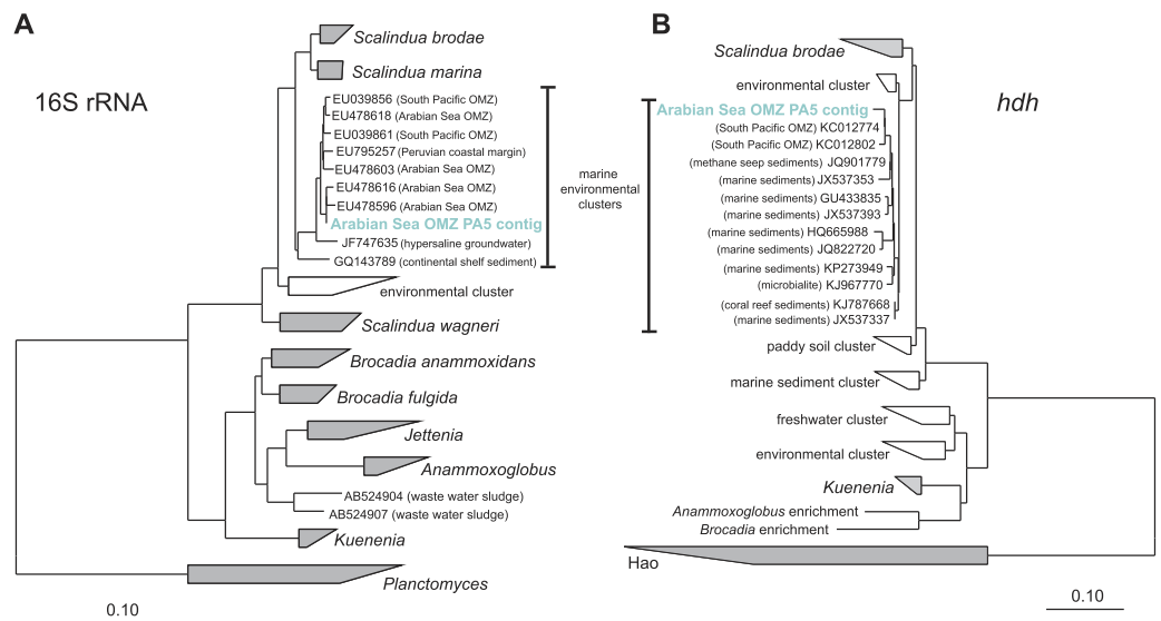
Figure 3 Phylogenetic inference of Scalindua -related contigs assembled from the OMZ metagenomes. The tree were calculated using the Neighbor Joining algorithm and based on 1,388 nucleotide positions for the 16S rRNA gene (A) and 180 deduced amino acid positions for the hydrazine dehydrogenase encoding gene ( hdh ) (B).
