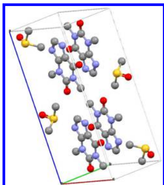
Figure 2. Unit cell of the theophylline DMSO solvate, from CSD (RIGYEM); hydrogens are omitted for clarity. DMSO is a borderline solvent, with a melting point of 19 °C.
