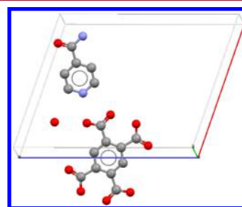
Figure 3. Asymmetric unit of protonated INA with a pyromellitic acid counterion and water, HEVPUU. This combination of a salt with a solvent molecule is not classifiable in the scheme presented in 8 Figure 1a.
