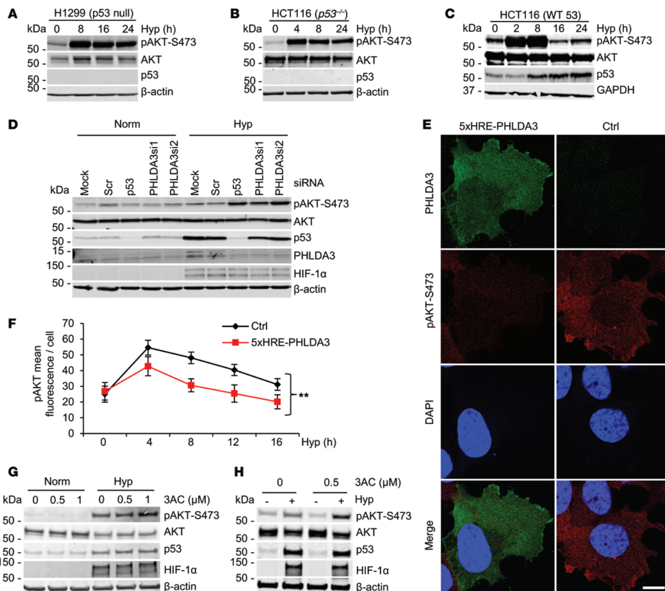
Figure 5. Hypoxia-induced activation of AKT is attenuated by p53/PHLDA3/SHIP-1 signaling. (A–C) Western blotting comparing AKT-S473 phosphorylation in H1299, HCT116 ( p53^{-/-} ), and WT HCT116 cells, respectively, exposed to hypoxia for the times indicated. (D) Western blotting for antibodies indicated in RKO cells transfected with either p53 or PHLDA3 siRNA and exposed to 8 hours of hypoxia. (E) Representative images of immunofluorescent staining with anti-PHLDA3 (green) and anti-pAKT-S473 (red) antibodies in H1299 cells transfected with 5xHRE-PHLDA3 or control and exposed to hypoxia for 12 hours. Scale bar: 10 \mu m. (F) Hypoxic time course for the mean intensity of pAKT-S473 fluorescence per cell in control or PHLDA3-expressing cells from E. The plot shows mean \pm SEM ( n = 3 , 2-way ANOVA test [ **P < 0.01 ]). (G) Western blotting in HCT116 cells exposed to 18 hours of normoxia or hypoxia in the presence or absence of SHIP-1 inhibitor, 3AC. (H) Western blotting in RKO cells exposed to 14 hours of normoxia or hypoxia in the presence or absence of 3AC.
