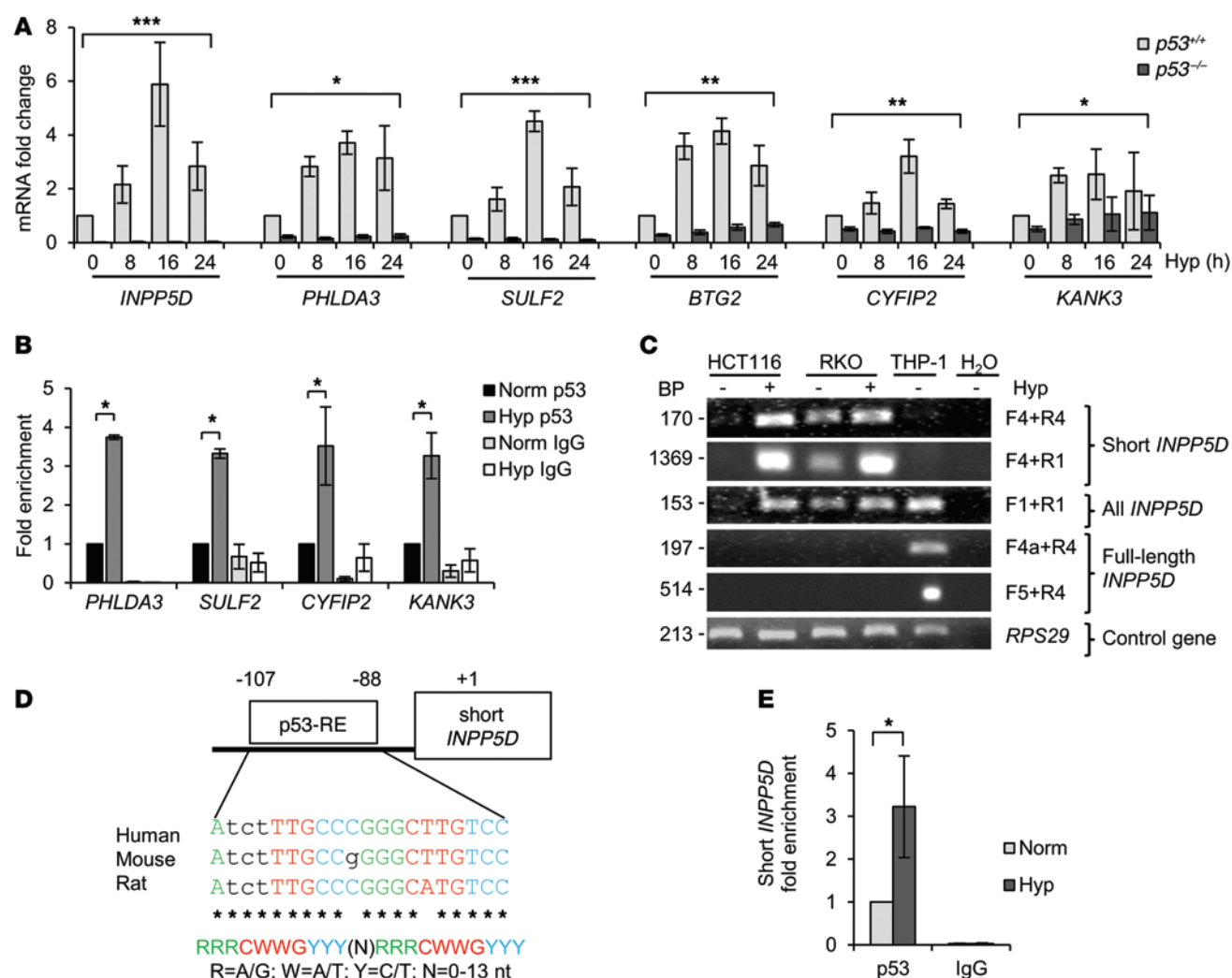
Figure 2. Transcriptional activity of p53 is required to induce expression of a specific group of genes in hypoxia. (A) Validation of p53 targets by qPCR in p53^{+/+} and p53^{-/-} HCT116 cells exposed to hypoxia. The bar graph shows mean \pm SEM (combined n = 3 , 2-way ANOVA test [ *P < 0.05 ; **P < 0.01 ; ***P < 0.001 ]). (B) qPCR for p53 ChIP in HCT116 cells exposed to 8 hours of normoxia or hypoxia for the genes indicated. The bar graph shows mean \pm SEM (combined n = 3 , 2-way ANOVA test [ P < 0.0001 ] followed by 2-tailed Student's t test [ *P < 0.05 ]). (C) PCR for the INPP5D transcripts using a combination of primers (marked as arrows in Supplemental Figure 2A) specifically detecting the short INPP5D transcript (F4+R4 or F4+R1), all INPP5D transcripts (F1+R1), or the full-length INPP5D transcript (F4a+R4 or F5+R4) on the cDNA from HCT116 or RKO cells exposed to 16 hours of hypoxia. THP-1 cDNA was used as a control for the expression of the full-length INPP5D . RPS29 is shown as a control gene. (D) Alignment of the putative p53 RE of the short INPP5D in human, mouse, and rat. A consensus p53 RE is shown below the alignment. (E) qPCR for p53 ChIP at the putative p53 RE in the short INPP5D promoter in HCT116 cells exposed to 8 hours of normoxia or hypoxia. The bar graph shows mean \pm SEM (combined n = 3 , 2-tailed Student's t test [ *P < 0.05 ]).
