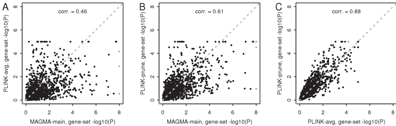
Fig 2. Comparison of self-contained gene-set analysis results. Gene set—log 10 p-values from the CD data self-contained gene-set analysis for MAGMA and PLINK. Panel (A) shows the PLINK-avg (no pruning) results compared with the MAGMA-main analysis, panel (B) the PLINK-prune results compared with the MAGMA-main analysis and (C) the two PLINK analyses compared to each other. P-values below 10 -8 are truncated to 10 -8 (grey points) to preserve the visibility of the other points.
