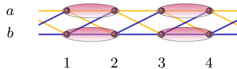
FIG. 6. Alternate Schwinger spin structure for the dual-rail quantum wire on periodic boundary conditions (where the number of Schwinger spins is even). Note that the qumodes are now paired horizontally into spins. A global nullifier for this state is illustrated by the purple ellipses, which denote the \hat{S}^z operator acting on all of the Schwinger spins in the system.
