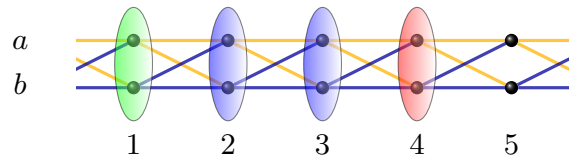
FIG. 4. A portion of the dual-rail quantum wire on periodic boundaries interpreted as a ring of Schwinger spins. The qumodes are paired vertically into Schwinger spins, labelled 1–5. The coloured ellipses are an illustration of the chain-like nullifier that results from taking linear positive combinations of three of the n independent nullifiers from Equation (5.3) (where the green and red ellipses correspond to \hat{S}_{1a,1b}^0 - \hat{S}_{1a,1b}^x and -\hat{S}_{4a,4b}^0 - \hat{S}_{4a,4b}^x respectively) and the 2\hat{S}^x operator acts on spins 2 and 3, indicated by the blue ellipses.
