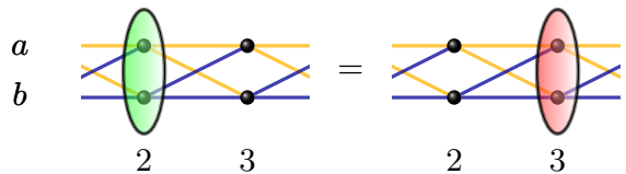
FIG. 7. Illustration of the local symmetry from (6.1). Applying e^{-i2\phi(\hat{S}_{2a,2b}^0 - \hat{S}_{2a,2b}^x)} (illustrated by the bold green ellipse) is equivalent to applying e^{-i2\phi(\hat{S}_{3a,3b}^0 + \hat{S}_{3a,3b}^x)} (illustrated by the bold red ellipse).
