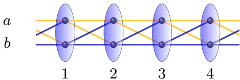
FIG. 5. Schwinger spin structure for the dual-rail quantum wire on periodic boundary conditions, where the qumodes (labelled by a and b ) are paired together vertically into Schwinger spins, labelled 1–4. The blue ellipses are an illustration of the global nullifier for this state—i.e., a \hat{S}^x operator acting on every Schwinger spin of the system.
