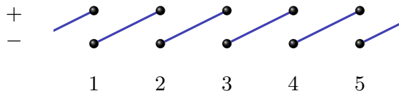
FIG. 3. The graph of the adjacency matrix for the dual-rail quantum wire in the distributed qumodes, with the qumode-operator relabelling (in terms of \pm along the vertical axis) as indicated in Equation (5.1). The weights of the links are all \tanh\alpha in this qumode decomposition.
