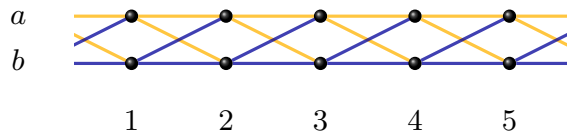
FIG. 2. The graph of the adjacency matrix ( \mathbf{K} ) for the dual-rail quantum wire on periodic boundary conditions. The weights of the links are \pm\frac{1}{2}\tanh\alpha , differentiated by the blue and yellow links, respectively. Schwinger spins are formed by pairing qumodes together vertically, where each Schwinger spin is labelled by integer values 1–5 and contains two qumodes, labelled by a and b .
