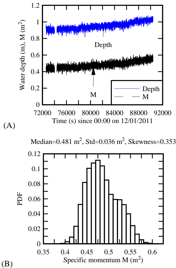
FIG. 7 – Instantaneous specific momentum M in Gardens Point Road on 12-13 January 2011 (tests T1 and T2, location A) - (A) Time variations of instantaneous water depth and specific momentum at location A during tests T1 and T2 - (B) Normalised probability distribution function of instantaneous specific momentum at location A during test T2
