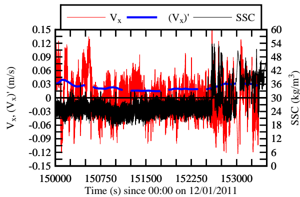
FIG. 5 – Time variations of the instantaneous longitudinal velocity component and suspended sediment concentration (SSC), and standard deviation of longitudinal velocity component at Gardens Point Road during on 13-14 January 2011 during the last sampling period T5
