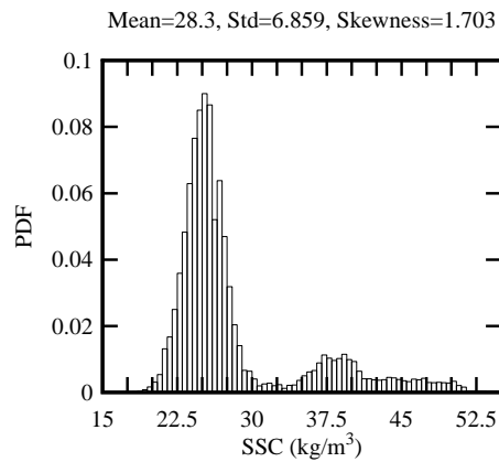
FIG. 6 – Normalised probability distribution function of instantaneous suspended sediment concentration (SSC) at Gardens Point Road during on 13-14 January 2011 during the last sampling period T5
