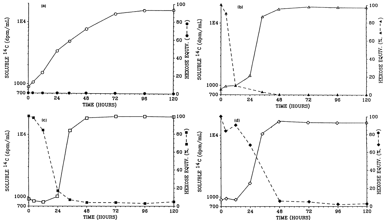
FIG. 4. The patterns of carbohydrate utilization by an anaerobic ruminal fungus grown on [U- 14 C]cellulose alone (a) or in combination with glucose (b), cellobiose (c), or starch (d). Disappearance of glucose, cellobiose, and starch was determined by the decline of the glucose concentration in culture fluids with time. The initial concentrations of glucose, cellobiose, and starch were determined by analysis to be 1.2, 1.9, and 3.0 g/liter, respectively.
