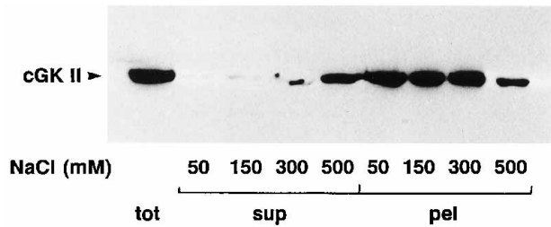
FIG. 1. Western blot demonstrating that solubilization of cGK II requires high salt in combination with Triton X-100. HEK 293 cells stably transfected with pRc/CMV-cGK II were homogenized and centrifuged at 20,000 × g to obtain a heavy membrane fraction which was then incubated with 1% Triton X-100 for 5 min at 0 °C in the presence of various concentrations of NaCl as indicated. Subsequently, samples were removed before and after centrifugation (15 min, 20,000 × g ) for detection of cGK II present in the total extract ( tot ) and supernatant ( sup ) and pellet ( pel ) fractions by immunoblotting. The results shown are representative of three experiments.
