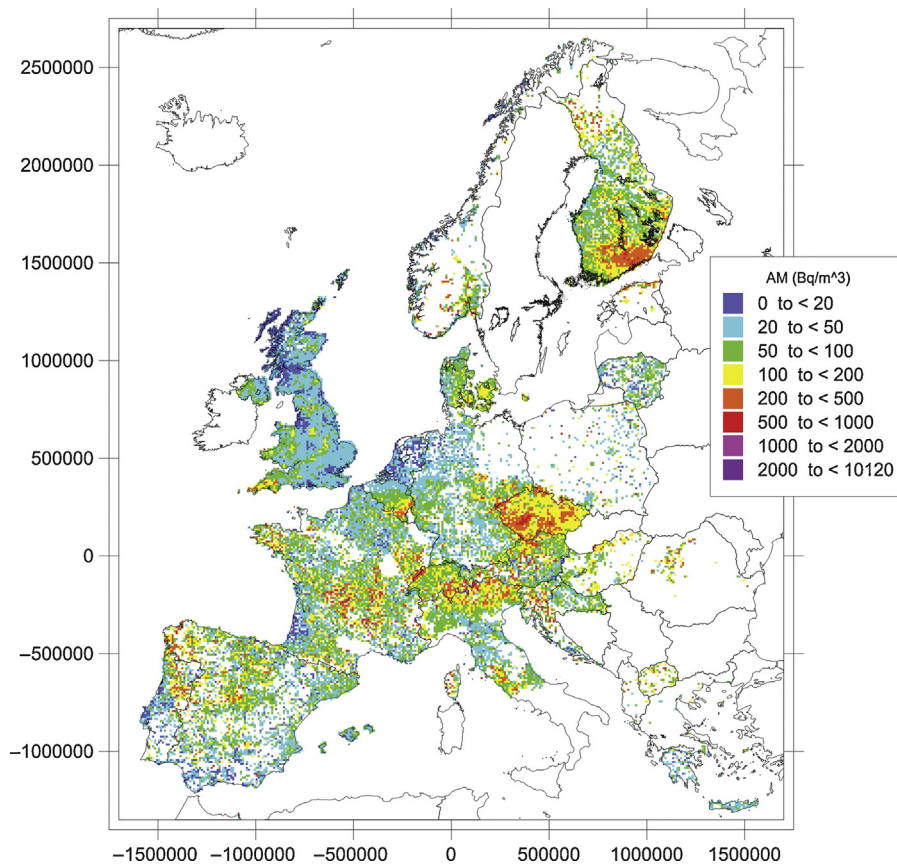
Fig. 4. Map of radon in Europe. Arithmetic means over 10 km × 10 km cells of long-term radon concentration in ground-floor rooms. Data available up until May 2014 included. Reproduced with permission of Oxford University Press [52].
