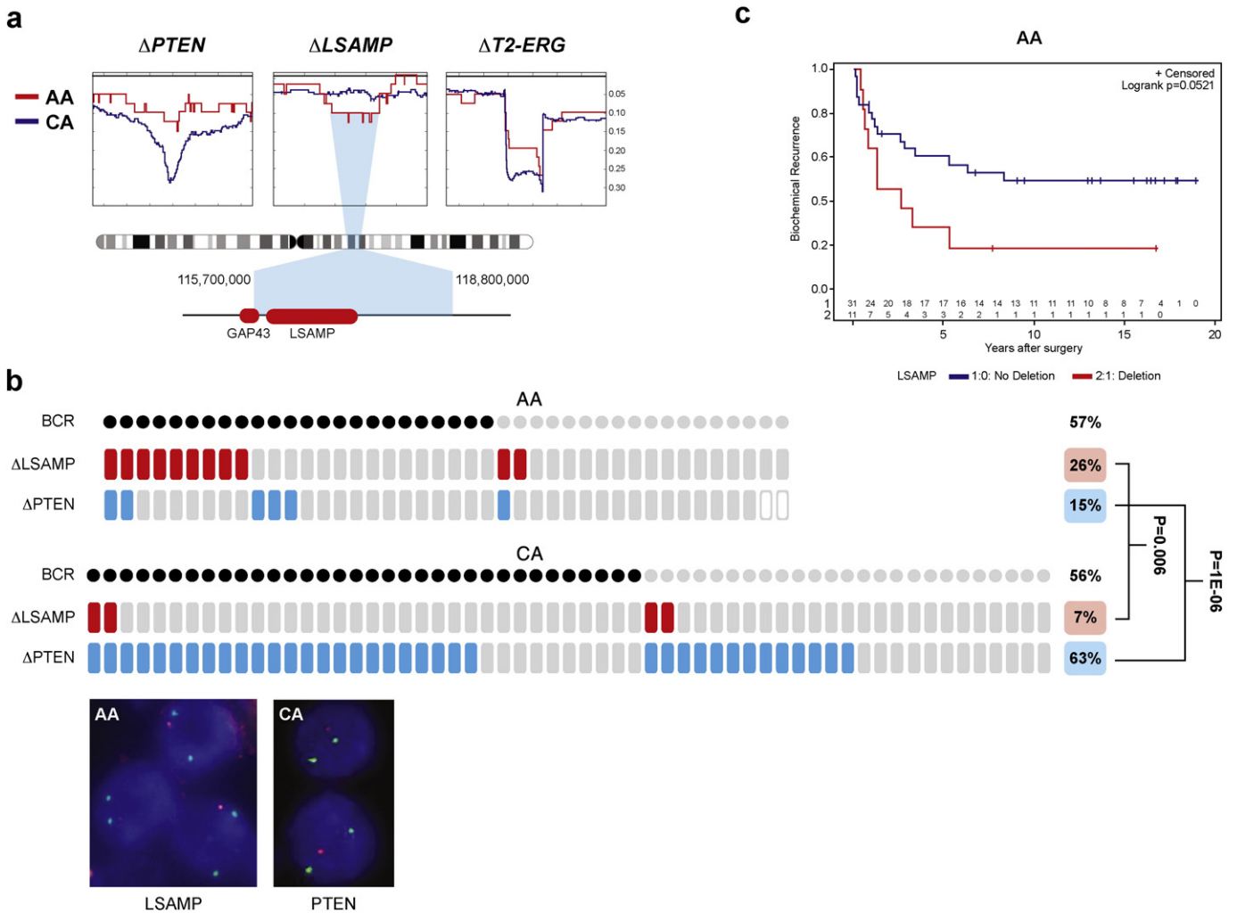
Fig. 3. LSAMP deletion is more prevalent in AA tumors correlating with rapid disease progression. Moreover, (a) SNP deletion frequencies in AA (red, n = 41) and CA (blue, n = 279) genomes indicate LSAMP within the minimum deletion region of 3q13.31 in AA patients. PTEN and TMPRSS2-ERG ( T2-ERG ) loci are more often deleted in CA patients. Deletion frequencies are marked on the Y-axis. (b) LSAMP deletion (red tiles) is associated with biochemical recurrence (BCR, marked by black dots) and is a more frequent event in AA patients. PTEN deletion (blue tiles) is a rare event in AA patients. Inset shows representative images of FISH assays of hemizygous LSAMP (red) and PTEN (red) deletions relative to centromeres (green), scale bar is 2 \mu m. (c) Rapid disease progression of AA patients harboring LSAMP deletion shown by the Kaplan–Meier biochemical recurrence free survival curves. Number of AA patients in BCR curves with deletion (red) or without deletion (blue) is marked above the X-axis.
