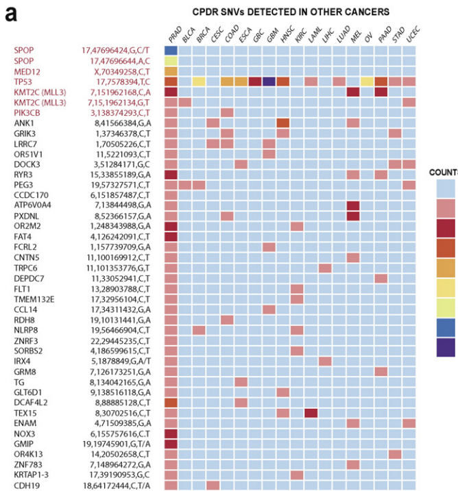
Fig. 1. Similarities and differences in the landscape of primary prostate cancer genomic alterations between AA and CA men. (a) Mutations identified in AA and CA genomes in this study are also found at higher frequencies in the TCGA prostate cancer mutation dataset (highlighted in red). (b) Affected loci or cytogenetic band (cb) of high confidence somatic structural variations (SV) and copy number variations (CNV) identified in AA or in CA genomes or in both ethnic group. Asterisk marks previously published somatic alterations.
