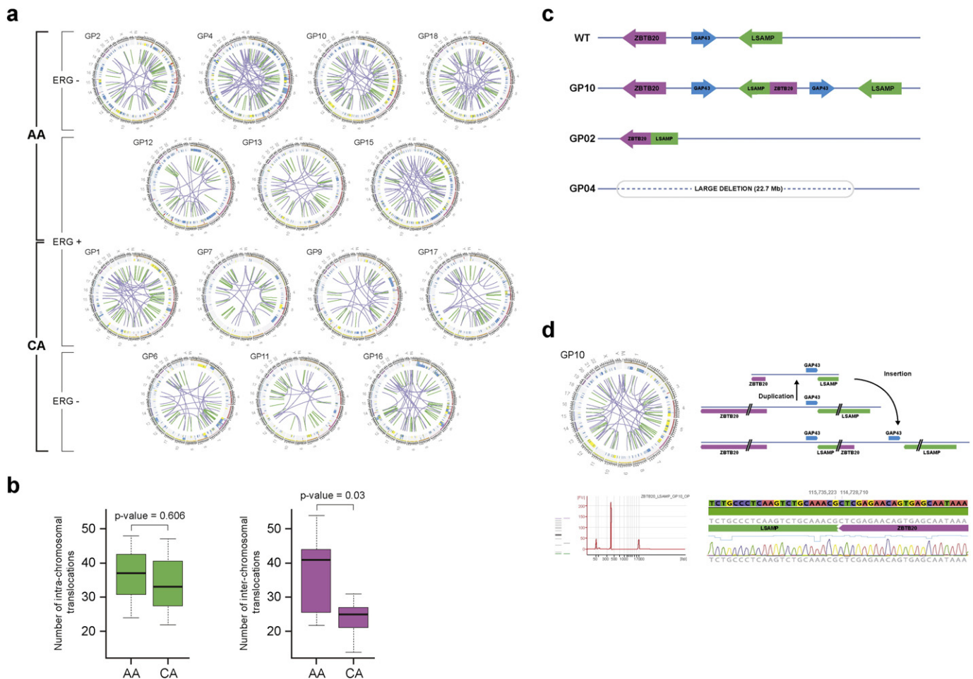
Fig. 2. Significantly higher number of inter-chromosomal rearrangements and exclusive association of chromosome LSAMP deletion/rearrangement in prostate cancer of AA men. (a) Circos plots of AA and CA whole genomes indicate chromoplexy characteristic of prostate cancer genomes. Inter-chromosomal translocations are marked with purple. Inter-chromosomal rearrangements are marked by green. (b) Inter-chromosomal translocations are significantly more frequent events in AA prostate cancer genomes. (c) Wild type (WT), LSAMP locus rearrangements by large deletion (patient GP04), small deletion (GP2) or by duplication generating a ZBTB20-LSAMP gene fusion (GP10). (d) Confirmation of ZBTB20-LSAMP gene fusion by Sanger sequencing of the genomic fusion junction.
