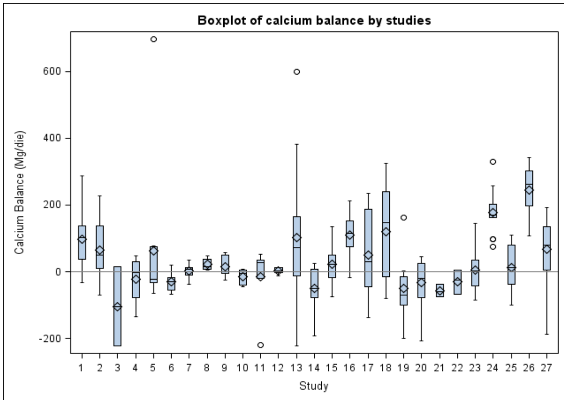
Figure 3: Boxplot of calcium balance by study
