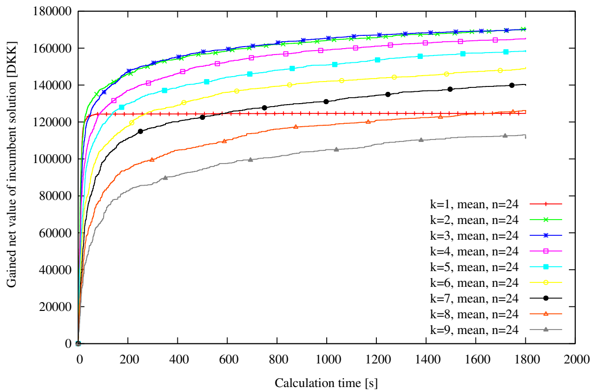
Figure 5: Convergence diagram for different values of k , i. e. the number of trajectories to remove and re-insert in one iteration. As may be seen, the best results are achieved with k = 3 . Each line represents the mean of n = 24 test runs.
