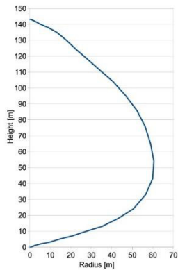
Figure 1: DeepWind optimized blade rotor.
