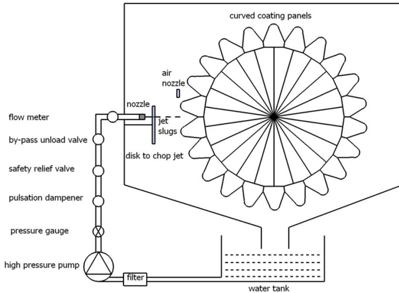
Figure 3.2 Schematic illustration of water jet erosion rig after modification with curved coating panels. Details of the setup are provided in [1].
