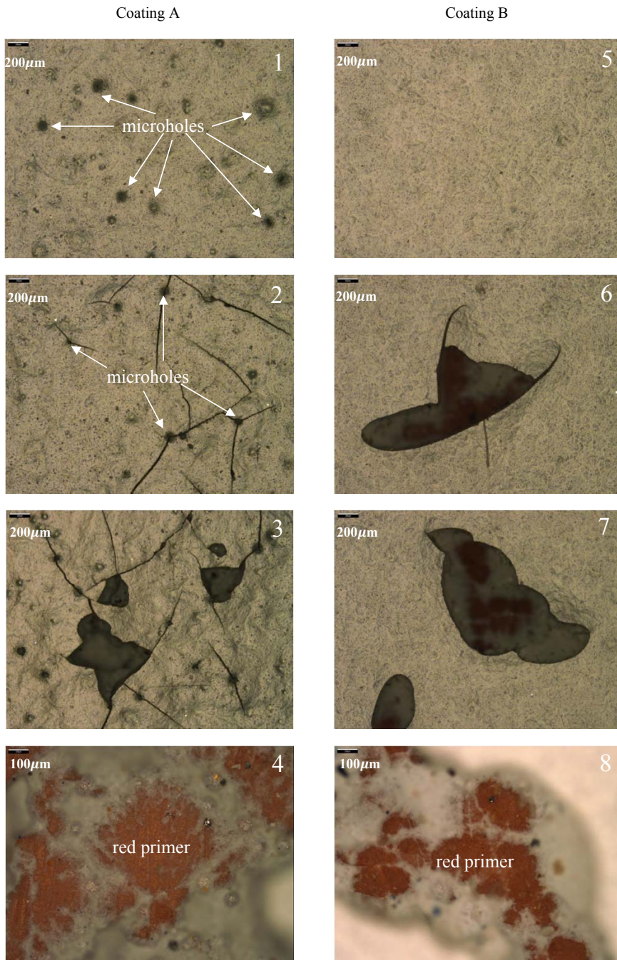
Figure 2.6 Microscopic photos of coating A after 30 seconds exposure and coating B after 10 minutes exposure using a continuous water jet. To the left, Coating A before (1) and after erosion (2-4) is shown. To the right, Coating B before (5) and after erosion (6-8) is seen.
