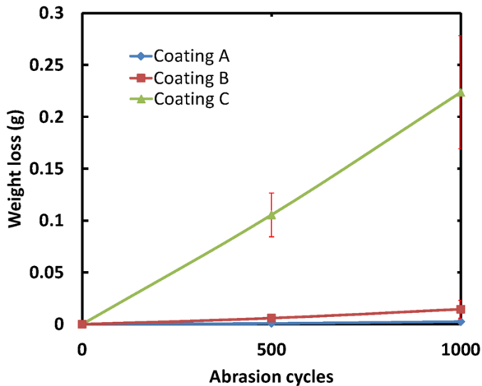
Figure 3.10 Weight loss data for the three blade coatings when exposed to abrasion cycles.
