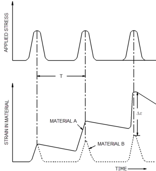
Figure 1.11 Relation between raindrop impact interval T and relaxation time, t , of elastomeric materials. After several impacts Material A, with t_A > T , reaches a strain \Delta\varepsilon greater than Material B, with t_B < T [51].
