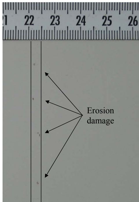
Figure 2.9 Photo of Coating A showing erosion damage after 60 hours. The scale is in centimeter. The area between the two solid lines was exposed to the water jet slugs.
