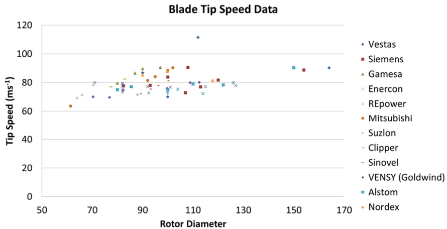
Figure 1.5 Blade tip speed versus rotor diameter for various utility scale wind turbine blades. Reproduced from [10].
