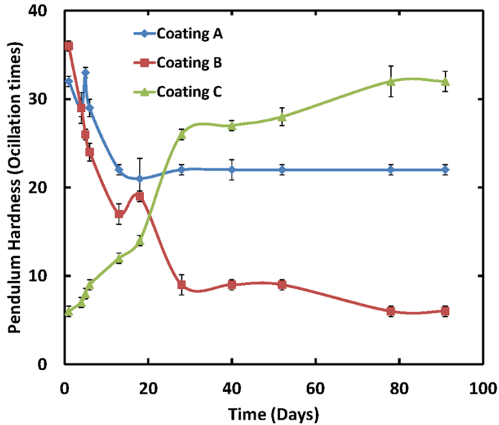
Figure 3.9 Measurements of pendulum hardness for the three blade coatings over time.
