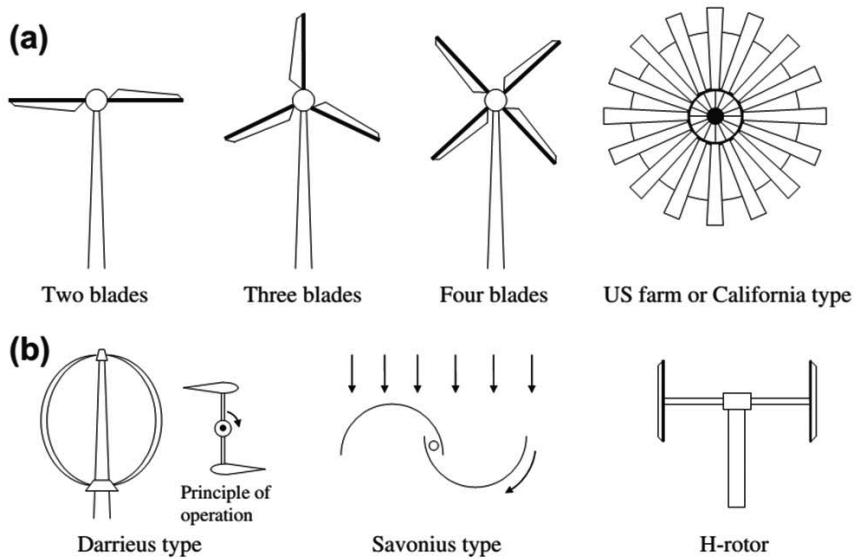
Figure 1.3 Wind turbine configurations. (a) Horizontal axis wind turbines. (b) Vertical axis wind turbines. Reproduced from [7].
