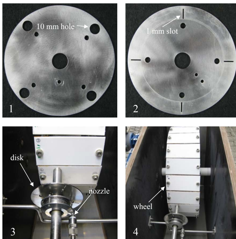
Figure 2.3 Disks with (1) 10 mm diameter holes and (2) 1 mm slots for chopping water jets. The smaller holes seen in the disk are used for fixation of the disk in the jet setup. Insert (3) shows the disk position in the rig and insert (4) the wheel with 22 coated panels.
