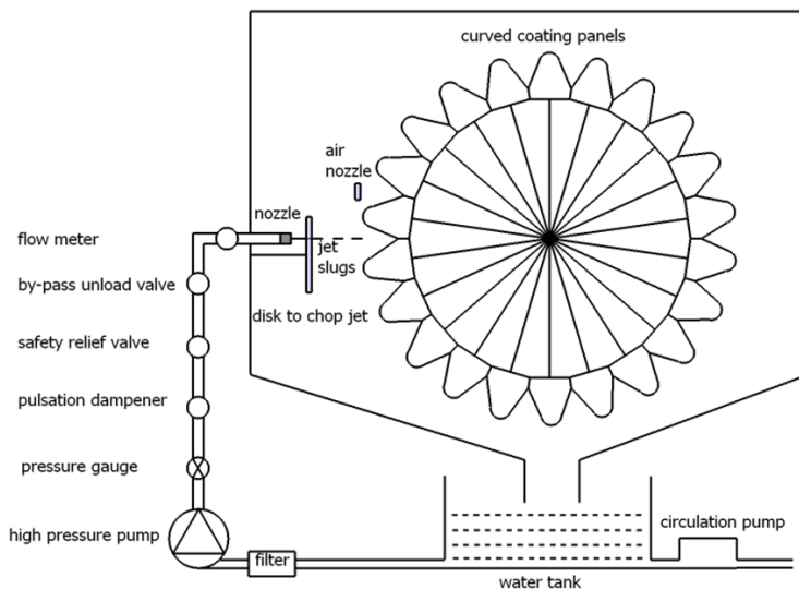
Figure 1 Schematic illustration (vertical cross-sectional view) of water jet erosion rig, including the disk, which ensures discrete water jets. The water recirculation tank holds about 50 liters of water.
