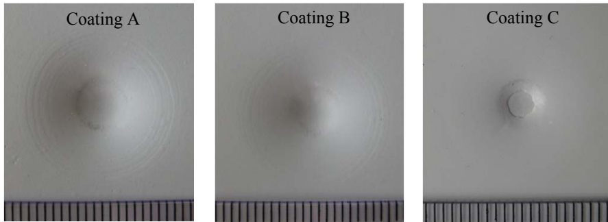
Figure 3.8 Digital camera photos of impact damages of the three non-exposed blade coatings. The scale at the bottom is 1 mm between two vertical lines.
