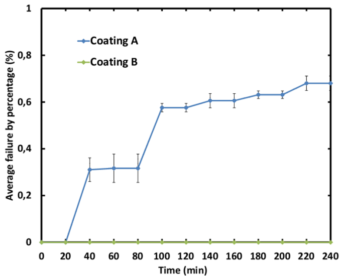
Figure 2.7 Experimental data of fraction of exposed coating area eroded in water jet setup. Standard deviations are shown as error bars. Coating B coincides with the x-axis.
