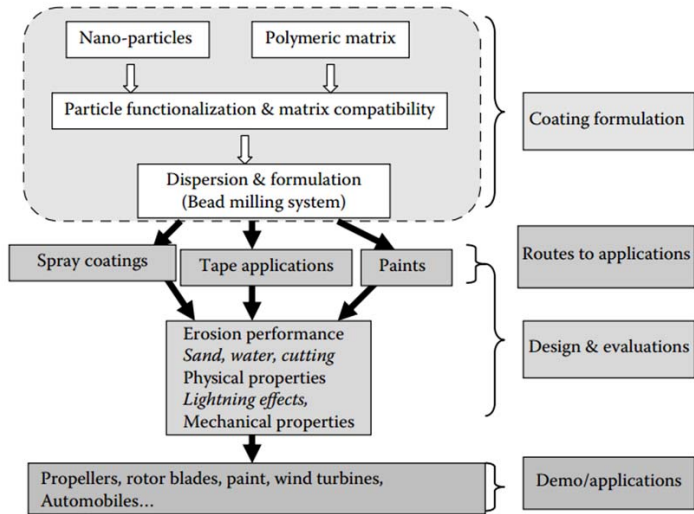
Figure 1.8 A proposed nanocomposite coating technology roadmap. Reproduced from [33].
