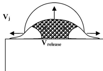
Figure 1.13 Droplet after shock wave has over-taken contact edge allowing decompression and jetting. V_j is jetting velocity. V_{\text{release}} is the release wave velocity. Reproduced from [37].
