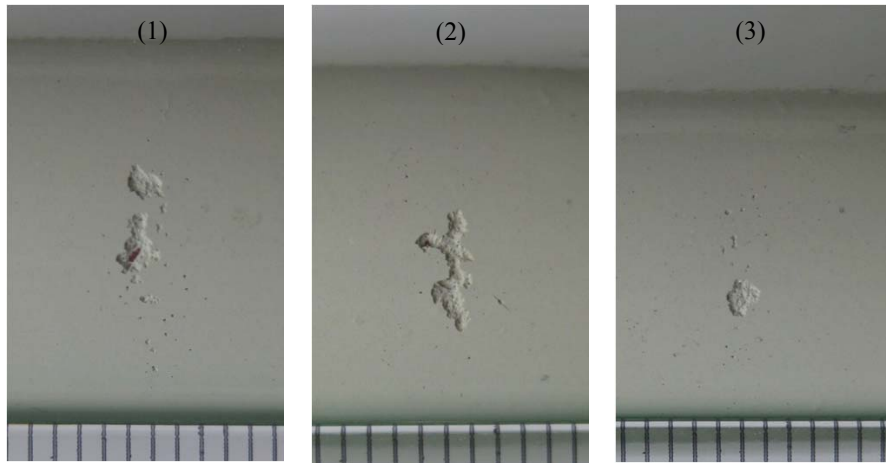
Figure 3.5 Digital camera photos of water jet erosion damage of Coating A when using curved panels (Experiment 3). Photos were taken after 30 minutes of experimentation. (1)-(3) refer to repetitions. The scale at the bottom is 1 mm between two vertical lines. In photo (1), the red underlying primer is visible in the large pit and the damage has penetrated the blade coating.
