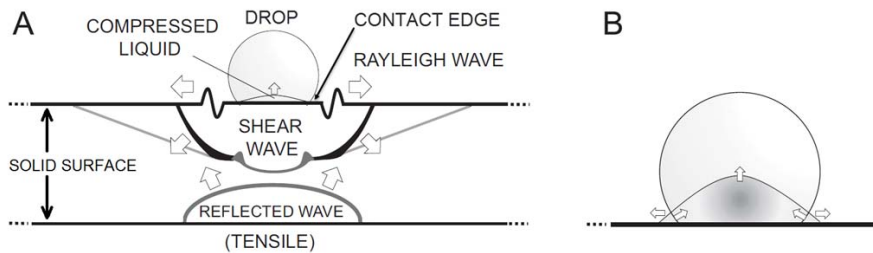
Figure 3.1 Schematic drawing of liquid droplet and rigid solid surface impact interaction. (A) shows the three main waves generated by the impact and (B) shows the deformation (outflow) of the compressed droplet. Reproduced from [8] with permission from Elsevier.
