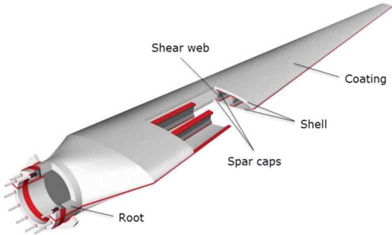
Figure 1.6 Wind turbine blade structure. The root is for connecting with wind turbine hub. The shell is to provide the aerodynamic shape and a structural role in stiffness and strength. The shear web and spar caps form the spar enhancing structure strength of a blade. The coating is for protecting the blade from environmental threats such as UV radiation and impacts from foreign bodies. Reproduced from [13].
