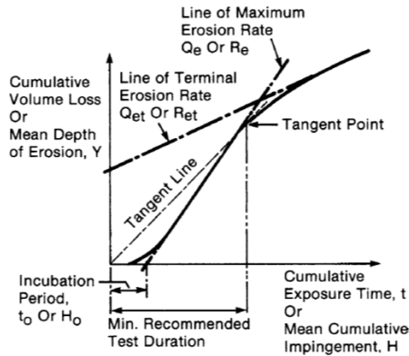
Figure 1.15 Cumulative erosion-time curve. Reproduced from [48].
