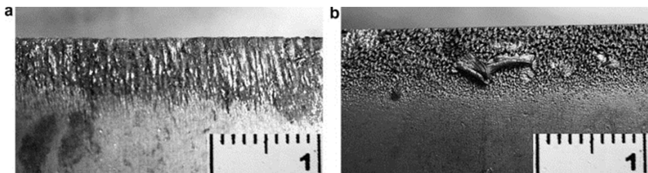
Figure 1.9 Steam turbine blade erosion. Reproduced from [39].
