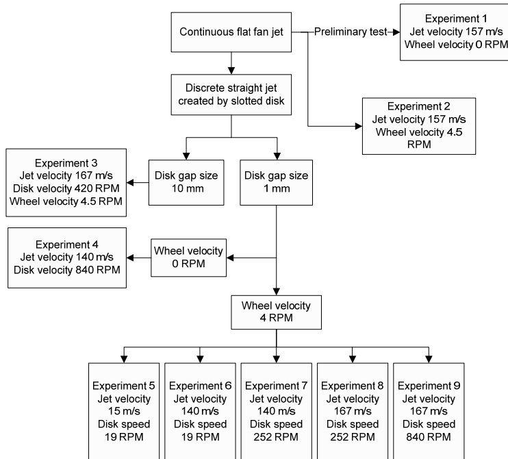
Figure 2.5 Overview of experiments conducted in the water jet setup. The chronological order of the experiments was from Experiment 1 - Experiment 9.
