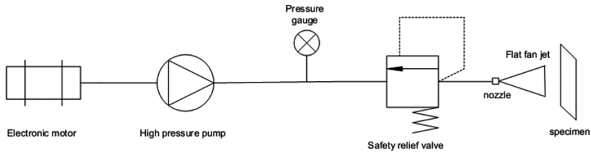
Figure 2.1 Rig V1- Schematic illustration of the continuous flat fan water jet erosion rig. Water for the jet is taken from a tank (not shown in figure) holding about 50 liters of water (no recycle was used).
