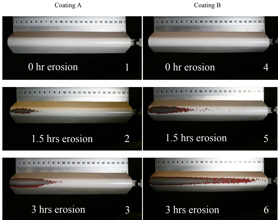
Figure 2.4 Results of rain erosion experiments in a whirling arm rig with two blade coatings. The highest impact velocity (rotor tip) was to the left on the panels, where erosion damage is most visible. The three left hand photos show Coating A before (1) and after erosion (2-3). To the right, Coating B, before (4) and after erosion (5-6), is seen. The scale shown in the figures is in cm.
