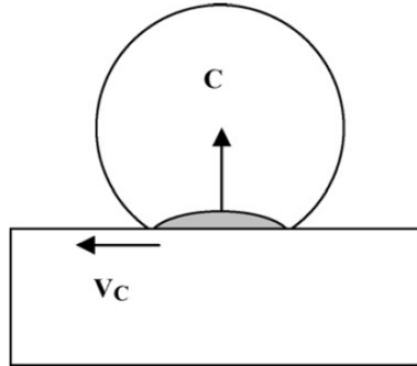
Figure 1.12 Droplet after initial impact: water drop is compressed due to lack of a free surface. V_C is the contact edge velocity. C is the shock wave velocity. Reproduced from [37].
