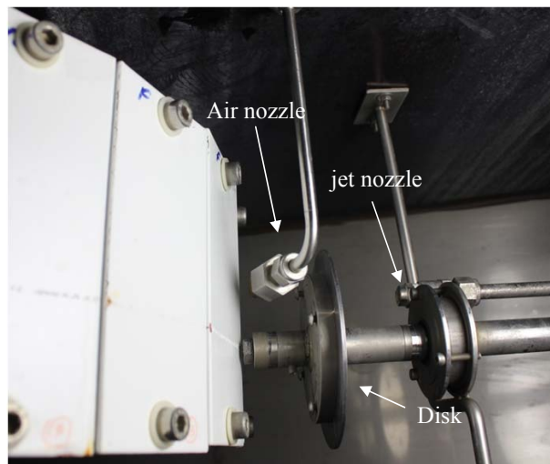
Figure 3.3 Photo showing the position of the air and water nozzles in the rig. The white panels to the left are blade coating samples attached to the large, slowly rotating, wheel.
