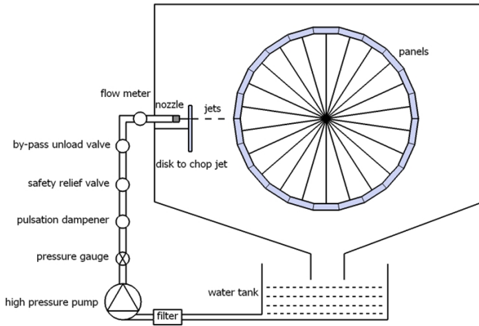
Figure 2.2 Rig V2 – Schematic illustration (vertical cross-sectional view) of water jet erosion rig, including the disk, which ensures discrete water jets. The water recirculation tank holds about 50 liters of water.
