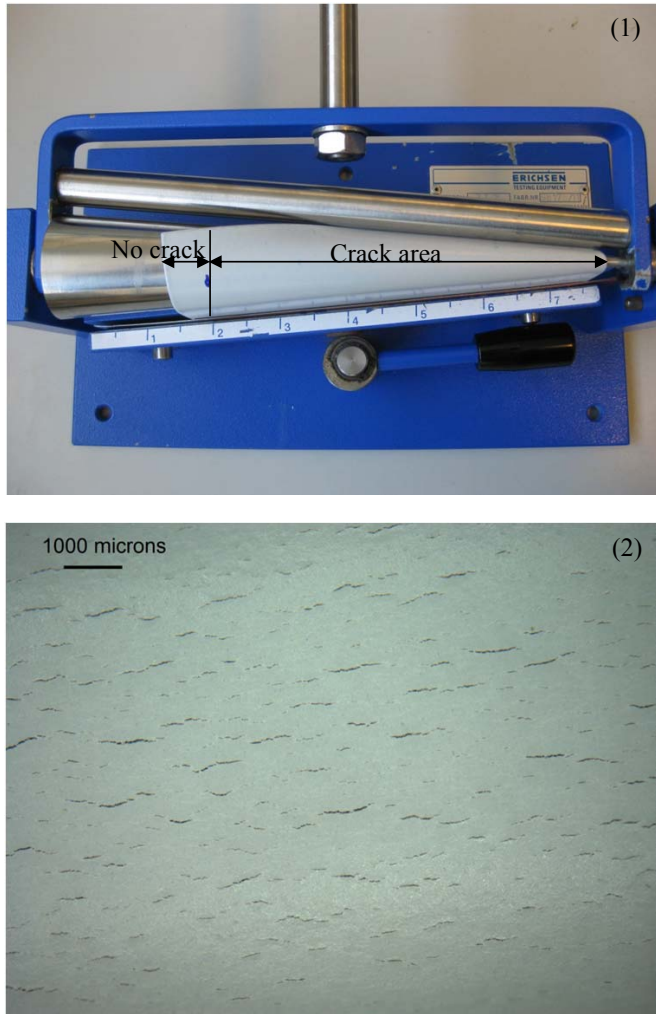
Figure 3.7 (1) Mandrel bending test equipment, (2) Optical microscopy of cracking of Coating C.
