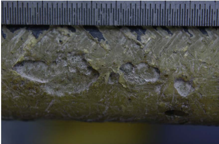
Figure 1.10 Erosion of the leading edge of a wind turbine blade removed from service. Leading edge dimensions shown are 44 mm horizontally and 20 mm vertically. Reproduced from [45].
