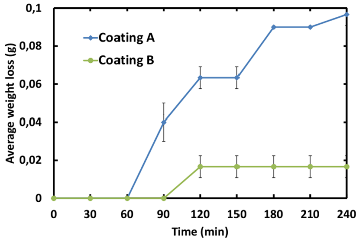
Figure 2.8 Experimental data of weight losses from coatings as a function of experimentation time. Standard deviations are shown as error bars.
