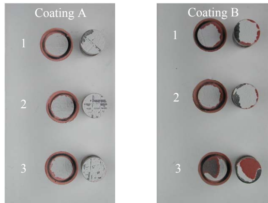
Figure 2.10 Photos showing results of pull-off adhesion experiments on non-exposed coatings. The bases of the detached dollies are shown to the right in each photo.
