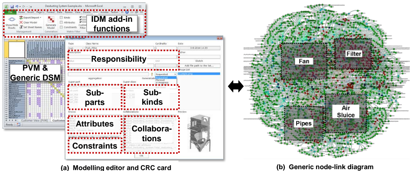
Fig. 6: IDM software tool showing (a) a collapsed generic DSM model and a CRC card, and (b) the generic node-link diagram on the example design problem
