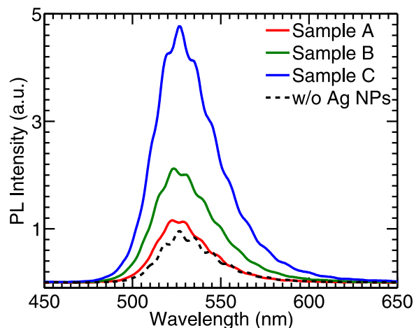
FIG. 3. Room temperature PL intensity of GaInN/GaN 5QWs with Ag NPs on top. Excitation power density is 756 W/cm 2 , and emission peak is around 530 nm.
