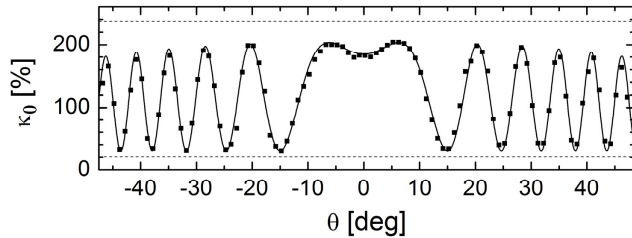
Fig. 9. Phase matched cascade enhancement \kappa_0 as a function of rotation angle of the phase plate around the vertical axis. Configuration 2, low power. Dashed lines: theoretically maximal and minimal \kappa . Points: measurements. Solid curve: theory normalized to the achieved maximum and minimum.
