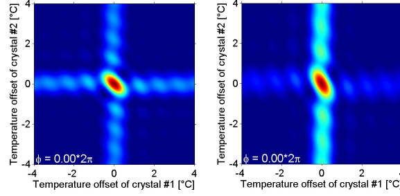
Fig. 2. Single-frame excerpts from the video illustrations in the online supplementary material which show the normalized N=2 cascade output power as a function of the two temperatures and the relative phase offset. Left: Configuration 1, where \eta_1 = \eta_2 (Media 1). Right: Configuration 2, where \eta_2 = 0.29 \times \eta_1 (Media 2).
