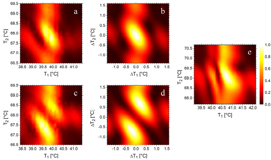
Fig. 11. Normalized output power from configuration 2 as a function of temperature set points of the two crystals, for various powers and phase plate settings. Linear interpolation is used between measurement points. The color scale shown in e applies to all plots. a : Low power measurement roughly at constructive interference. b : Simulation with \phi = 0 . c : Low power measurements roughly at destructive interference. d : Simulation with \phi = \pi . e : Measurement at maximum input power and constructive interference.
