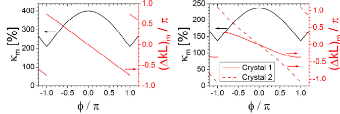
Fig. 3. Simulated temperature-optimized enhancement factor and the optimal \Delta k L values as a function of relative phase offset in a two-crystal cascade. Left: Two identical crystals, \eta_1 = \eta_2 , as in cascade configuration 1. In this case, (\Delta k_1 L_1)_m = (\Delta k_2 L_2)_m . Right: The case where \eta_2 = 0.29 \times \eta_1 , as in cascade configuration 2.
