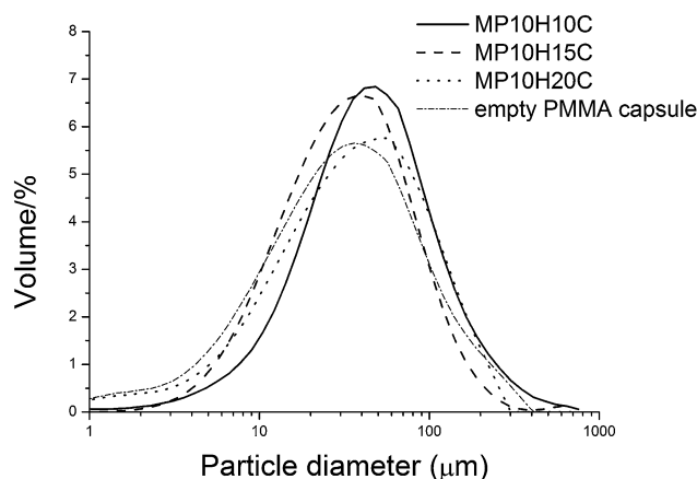
Fig. 3 Size distribution of MP10H10C, MP10H15C, MP10H20C microcapsules and empty PMMA capsules.
