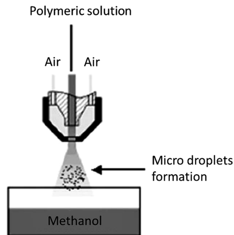
Fig. 1 Schematic diagram of the spraying setup.
