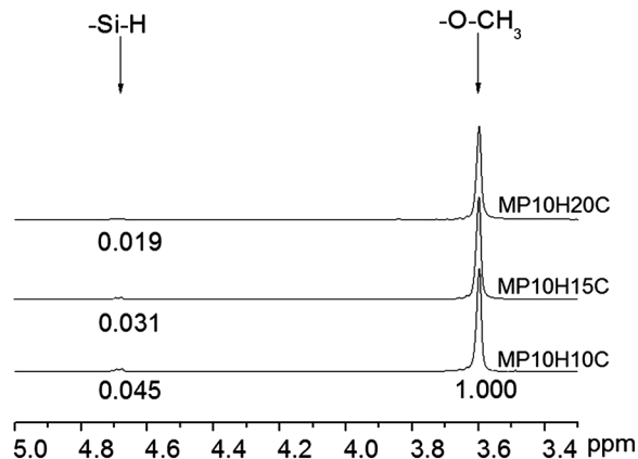
Fig. 4 ^1\text{H} NMR spectra of MP10H10C, MP10H15C and MP10H20C microcapsules with an indication of the characteristic peaks for Si-H and -O-CH 3 .
