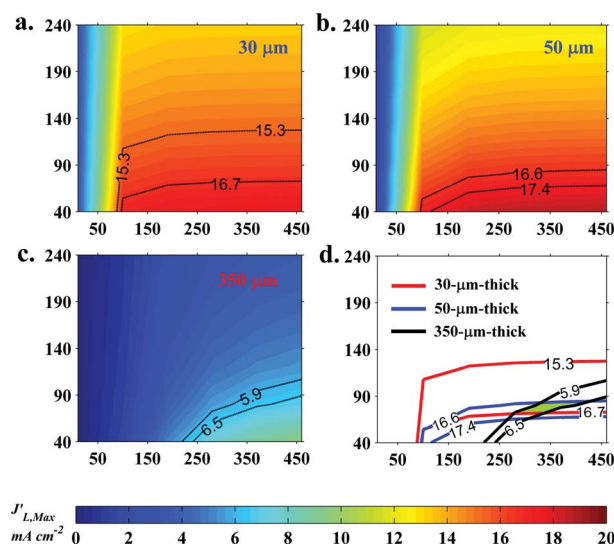
Fig. 9 Contour plot of theoretical maximum current density versus diffusion length and surface recombination rate under simulated illumination (Fig. 6) considering reflectance from the surface of the back side versus diffusion length and surface recombination rate for 30 \mu\text{m} thick (a), 50 \mu\text{m} thick (b), 350 \mu\text{m} thick (c). Overlapped contour lines (d) which correspond to the experimental uncertainty are also given to estimate diffusion length and surface recombination rate of the samples used for this work. Uncertainty ranges for each panel were derived from the uncertainty of the saturated current I_L and the active area measurement A , i.e. I_L/A \pm (\Delta I_L + \Delta A) .
