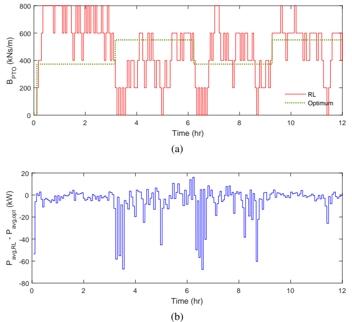
Fig. 12. Optimal and RL-control-selected ( J = 1 , K = 4 , L = 5 ) PTO damping coefficient (a) and corresponding mean absorbed power (b) in irregular waves with four sea states, generated from the combination of H_s = 2, 3 m and T_z = 7, 8 s.
