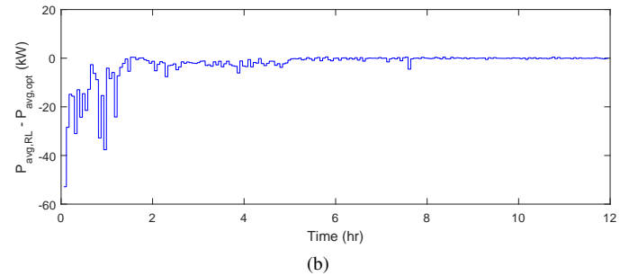
Fig. 10. RL-control-selected and optimal PTO damping coefficient (a) and difference in the corresponding mean absorbed power (b) in irregular waves with H_s = 2 m and T_z = 7 m, generated using a JONSWAP spectrum.
