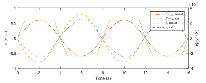
Fig. 9. PTO velocity and force over two wave periods in regular waves with H_s = 2 m and T_z = 8 s for the cases of unsaturated ( B_{PTO} = 300 kNs/m) and saturated ( B_{PTO} = 800 kNs/m) PTO force, when F_{Max} = 237.910 kN.
