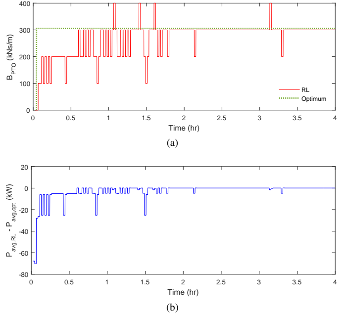
Fig. 7. RL-control-selected and optimal PTO damping coefficient (a) and difference in the corresponding mean absorbed power (b) in regular waves of unit amplitude and a wave period of 8 s.
