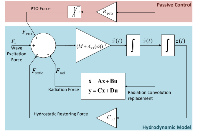
Fig. 2. Block diagram used for the calculation of the motion of the float.
