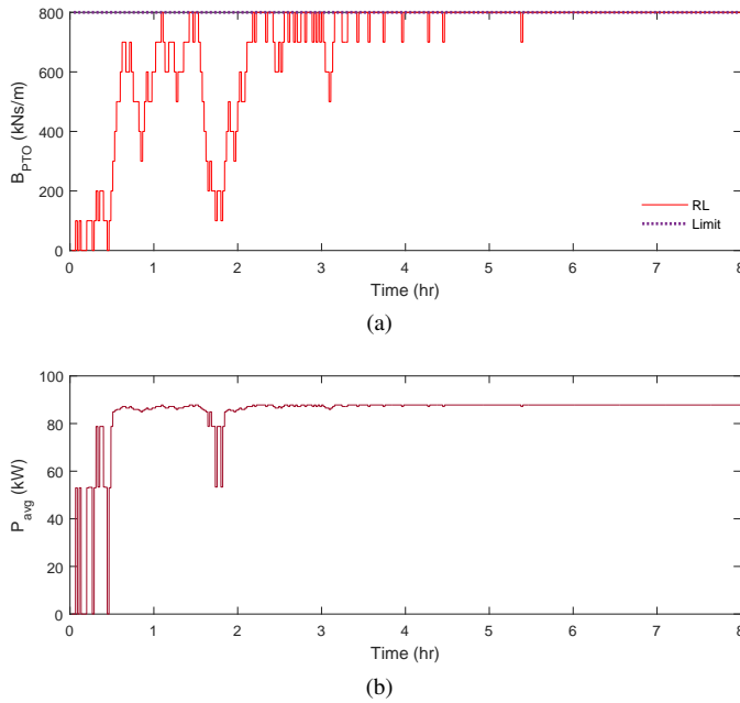
Fig. 8. RL-control-selected PTO damping coefficient (a) and corresponding mean generated power (b) in regular waves with H_s = 2.2 m and T_z = 8 s, when F_{Max} = 237.910 kN.
