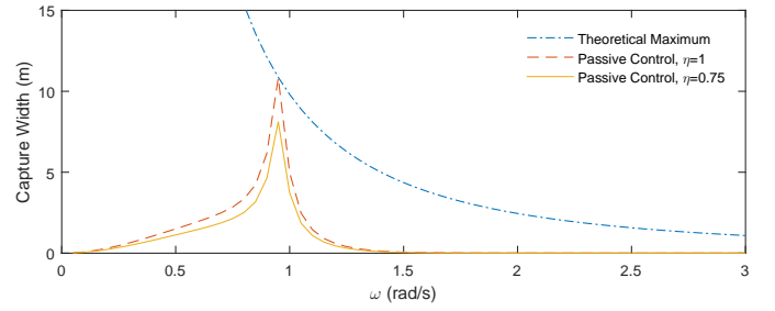
Fig. 3. Performance of a point absorber using passive control with two PTO efficiency values as compared with the case of theoretical maximum power absorption.
