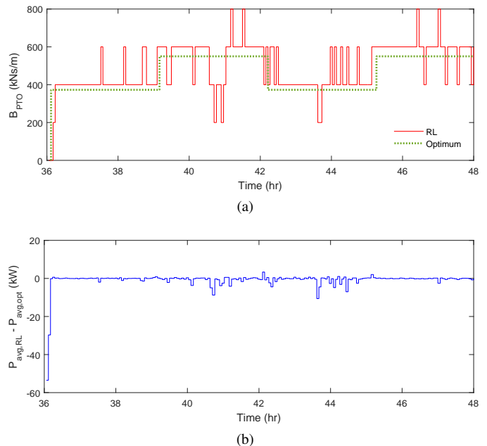
Fig. 13. Optimal and RL-control-selected ( J = 1 , K = 4 , L = 5 ) PTO damping coefficient (a) and corresponding mean absorbed power (b) in irregular waves with four sea states, generated from the combination of H_s = 2, 3 m and T_z = 7, 8 s after learning has occurred.
