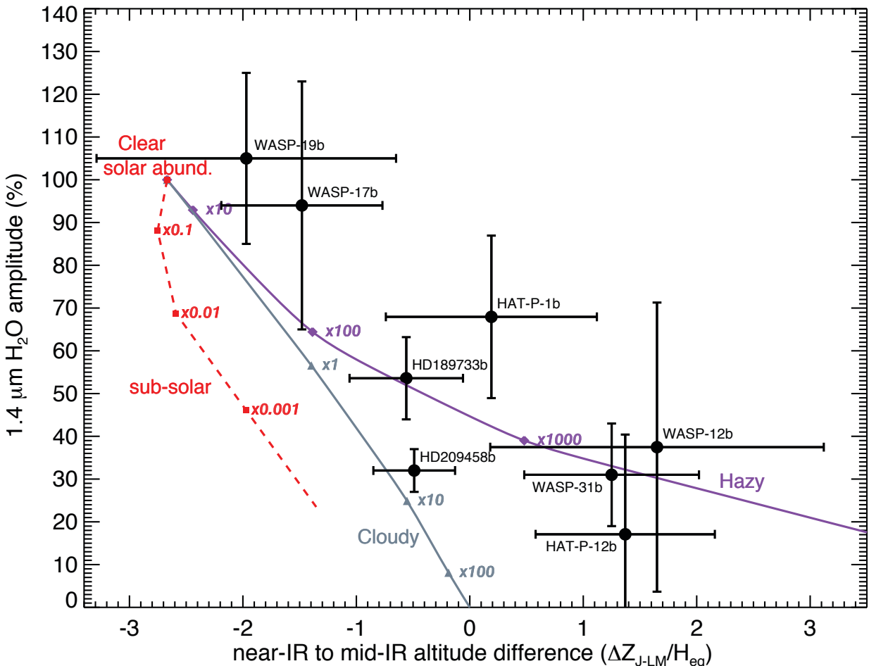
Figure 3 | Transmission spectral index diagram: \Delta Z_{\text{J-LM}} vs. \text{H}_2\text{O} amplitude. Black points show the altitude difference between the near-infrared and the mid-infrared spectral features ( \Delta Z_{\text{J-LM}} ) vs. the amplitude of the 1.4 μm \text{H}_2\text{O} feature for eight of ten targets (see Table 1). Error bars represent the 1\sigma measurement uncertainties. Purple and grey lines show model trends for hazy and cloud atmospheres, respectively, with increasing Rayleigh scattering haze and grey cloud deck opacity corresponding to 10x, 100x, and 1,000x solar. We also show clear-atmosphere models with sub-solar
