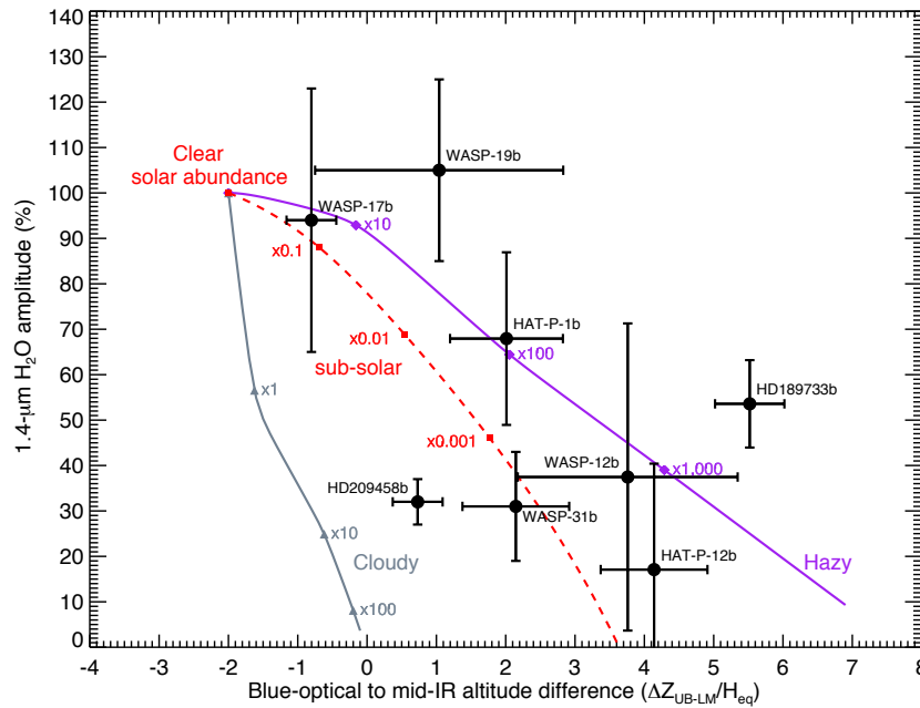
Extended Data Figure 2 | \Delta Z_{UB-LM} index vs. H_2O amplitude. Black points show the altitude difference between the blue-optical and mid-infrared spectral features ( \Delta Z_{UB-LM} ) vs. the amplitude of the 1.4\ \mu m H_2O absorption spectral feature (see Table 1). Error bars represent the 1\sigma measurement uncertainties. Purple and grey lines show model trends for hazy and cloud atmospheres, respectively, with increasing Rayleigh scattering haze and grey cloud deck opacity corresponding to 10x, 100x, and 1,000x solar. We also show clear-atmosphere models with sub-solar abundances of 0.1x, 0.01x and 0.001x solar (red line).
