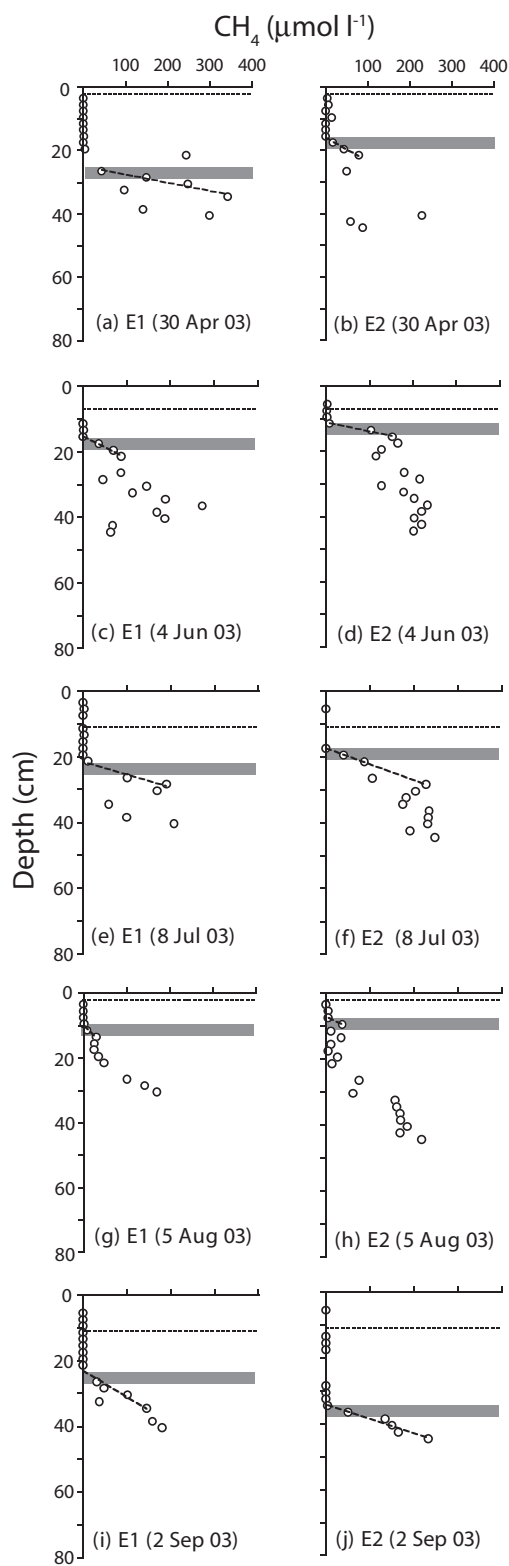
Fig. 5. Pore water profiles of dissolved \text{CH}_4 measured at Blaen Ffyn during the summer of 2003 from pore water equilibrators E1 and E2. Legend details are the same as described in the caption of Fig. 3.
