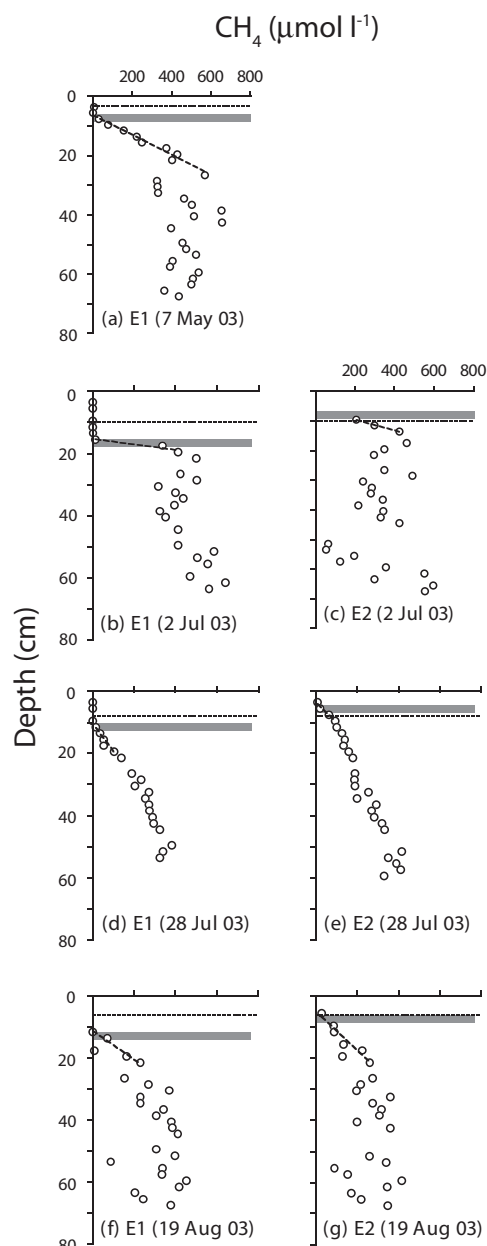
Fig. 3. Pore water profiles of dissolved \text{CH}_4 measured at Crymlyn Bog during the summer of 2003 from pore water equilibrators E1 and E2. Water-table level in each panel is indicated by a dotted horizontal line and inverted filled triangle. The dashed line through shallow \text{CH}_4 values trending to zero concentration is a regression line fitted to the data to determine the gradient d[\text{CH}_4]/dz , which was used to calculate rates of \text{CH}_4 flux into the methanotrophic zone and the depth at which [\text{CH}_4] = 0 \mu\text{mol l}^{-1} (i.e., the y-intercept denoted as [\text{CH}_4]_0 ). The gray horizontal bar delineates a 3 cm thick zone immediately beneath depth [\text{CH}_4]_0 in which potential rates of \text{CH}_4 oxidation were calculated based upon experimentally determined kinetic parameters (see Sect. 4.3) and in situ dissolved \text{CH}_4 concentrations. If gaps existed in pore water [\text{CH}_4] data, missing values were interpolated between adjacent \text{CH}_4 concentrations, including when necessary the point [\text{CH}_4]_0 = 0 \mu\text{mol l}^{-1} .
