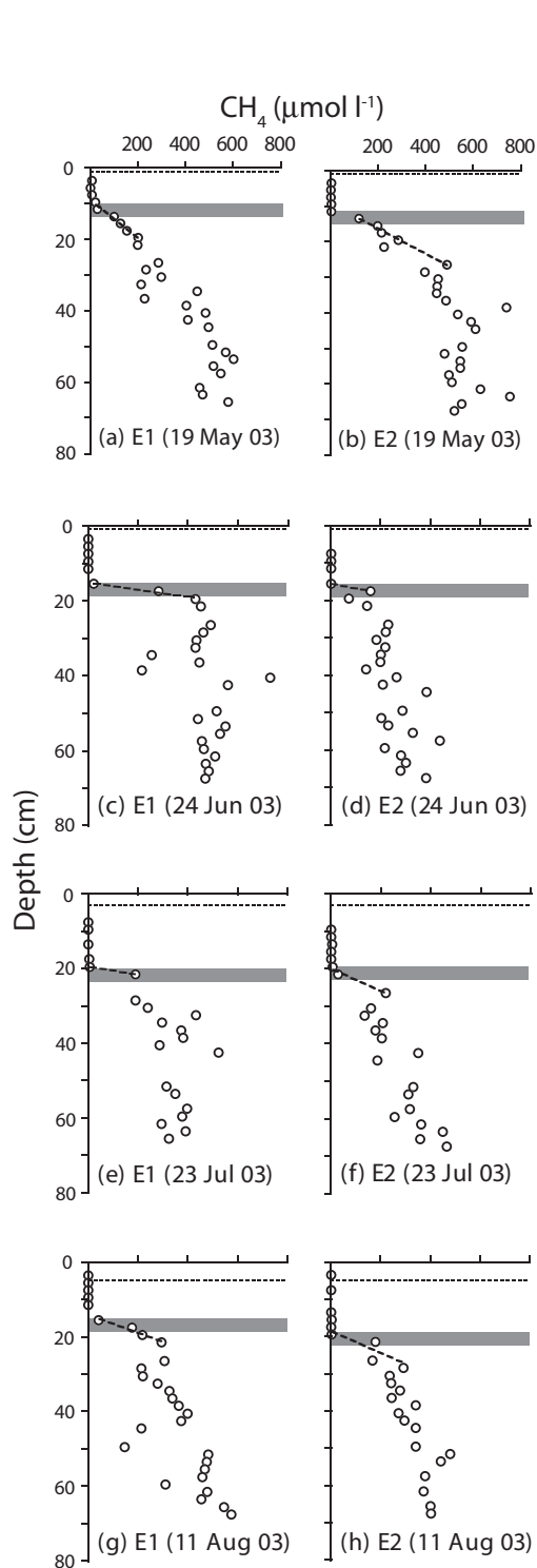
Fig. 4. Pore water profiles of dissolved \text{CH}_4 measured at Gors Lwyd during the summer of 2003 from pore water equilibrators E1 and E2. Legend details are the same as described in the caption of Fig. 3.
