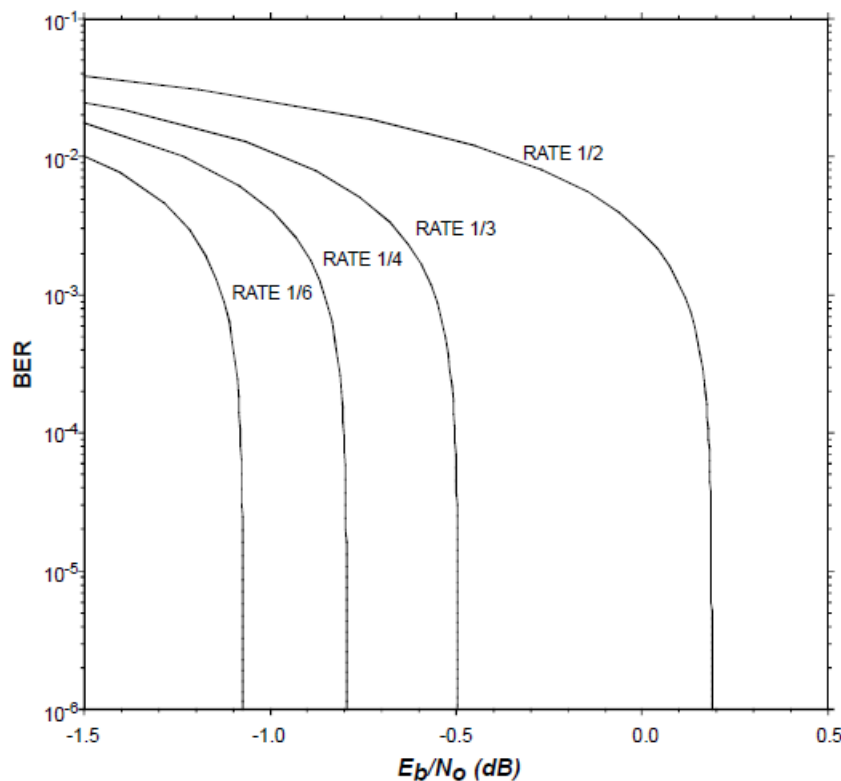
Figure 104: Capacity limits on the BER performance for codes with different rates operating over a binary input AWGN channel [62]
