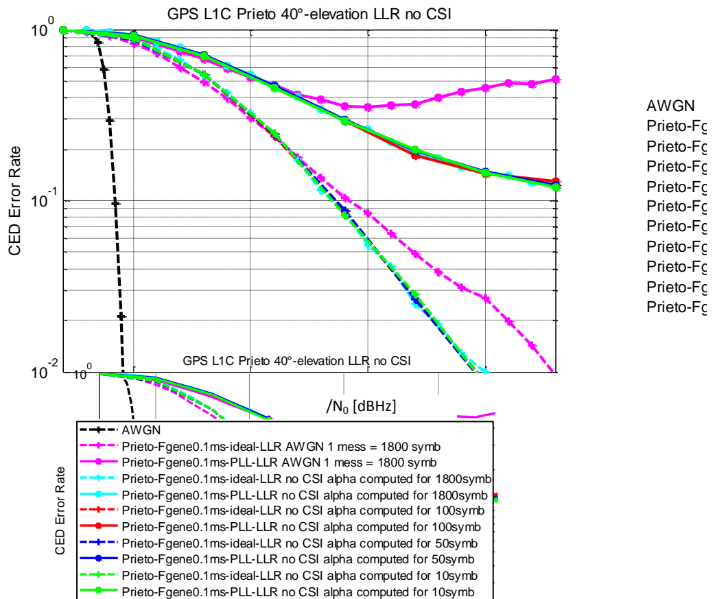
Figure 81: GPS L1C demodulation performance obtained with LLR_{no\ CSI} in the Prieto channel model
