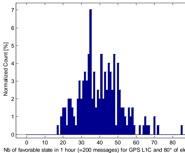
Figure 60: ‘Favorable state messages’ histogram, for GPS L1C in the Prieto channel model with 80^\circ of elevation considering the Prieto channel GOOD states as favorable reception conditions
