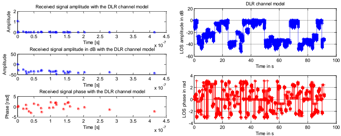
Figure 43: a) DLR channel model CIR example, with 90^\circ of azimuth angle - b) Amplitude and phase of the DLR channel model simulated samples, with 90^\circ of azimuth angle
