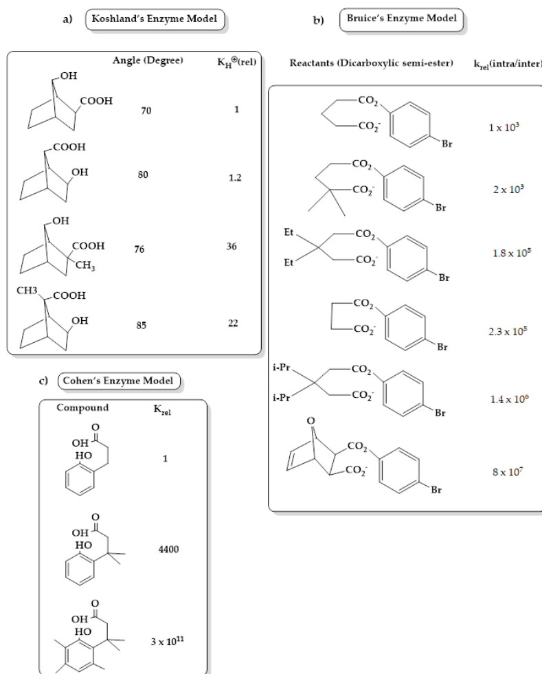
Figure 1. (a) Principles of “orbital steering” theory by Koshland, which describe the relative reactivity of lactonization of some hydroxy acids [47]; (b) acceleration rates of cyclization of di-carboxylic semi-esters of Bruice’s system [48]; (c) Cohen enzyme model of stereopopulation control, which describes the relative reactivity of lactonization of some hydroxyhydrocinnamic acids [47].
