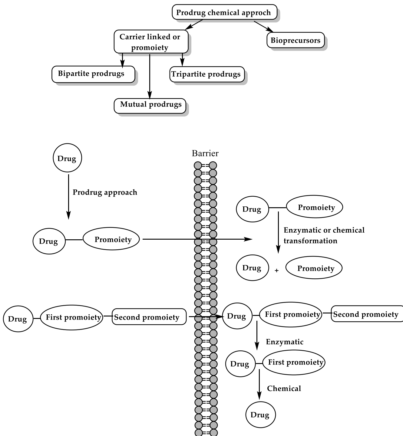
Figure 4. Classification of the chemical prodrug approach and its concept of transformation inside the body.
