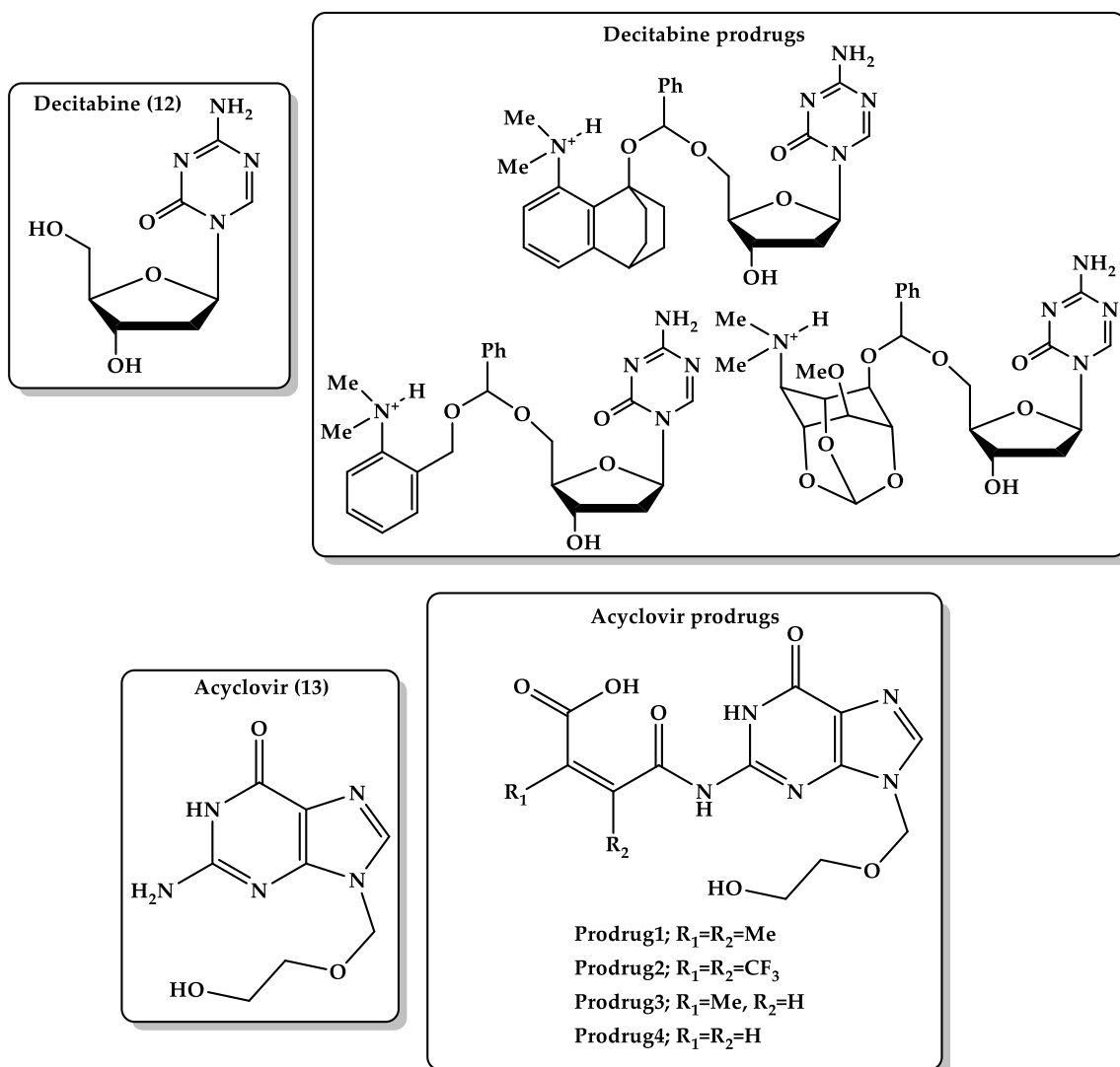
Figure 9. Chemical structures of decitabine (12) and its prodrugs and acyclovir (13) and its prodrugs.
