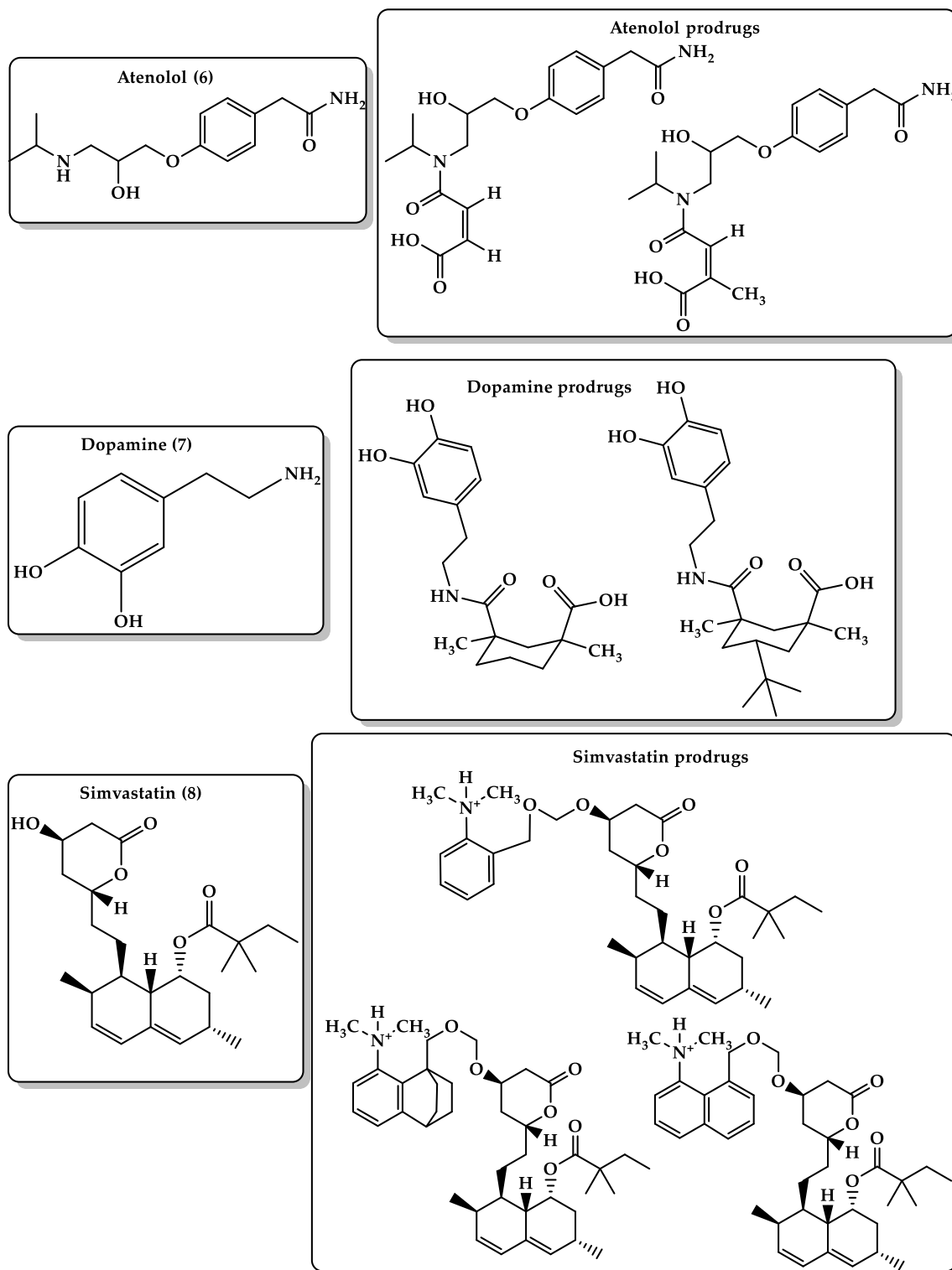
Figure 7. Chemical structures of atenolol (6) and its prodrug, dopamine (7) and its prodrugs, and simvastatin (8) and its prodrugs.
