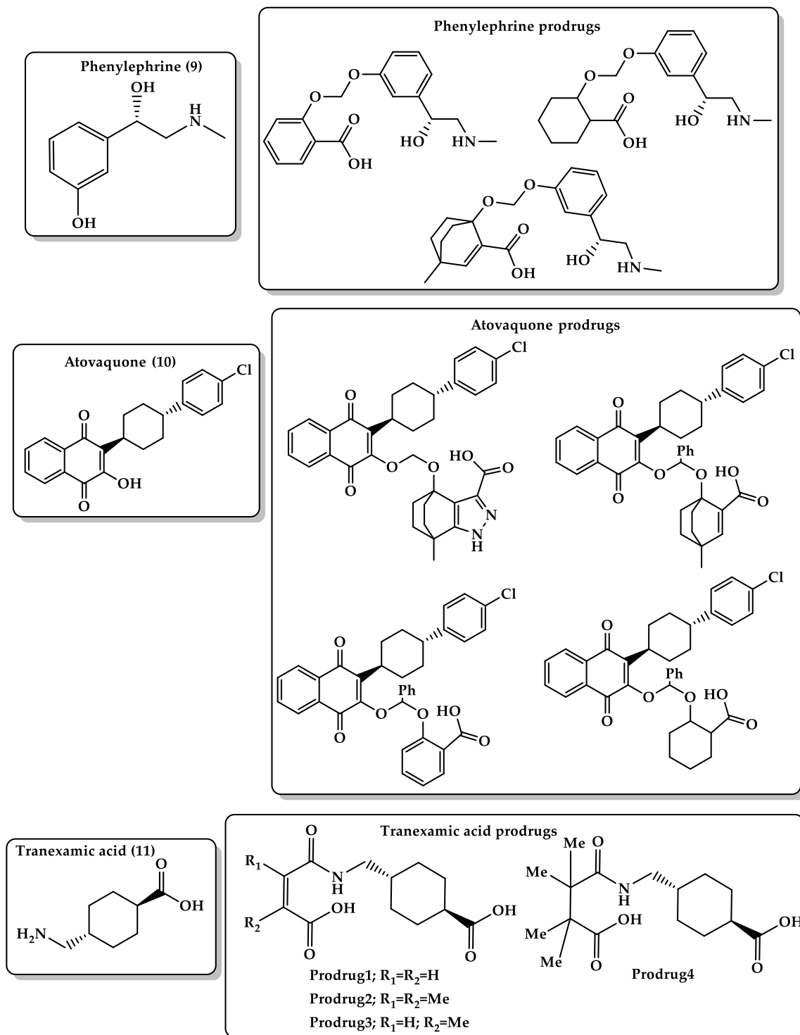
Figure 8. Chemical structures of phenylephrine (9) and its prodrugs, atovaquone (10) and its prodrugs, and tranexamic acid (11) and its prodrugs.
