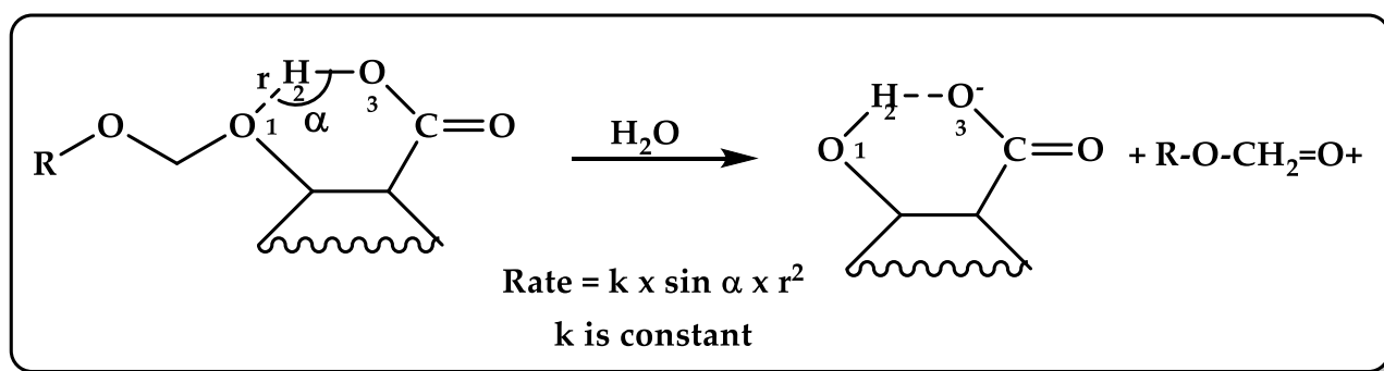
Figure 2. Proton transfer in Kirby's enzyme model where \alpha is the angle of attack O1H2O3 and r is the distance between the two reacting centers, H2–O1. R is an alkyl or aryl group [57].
