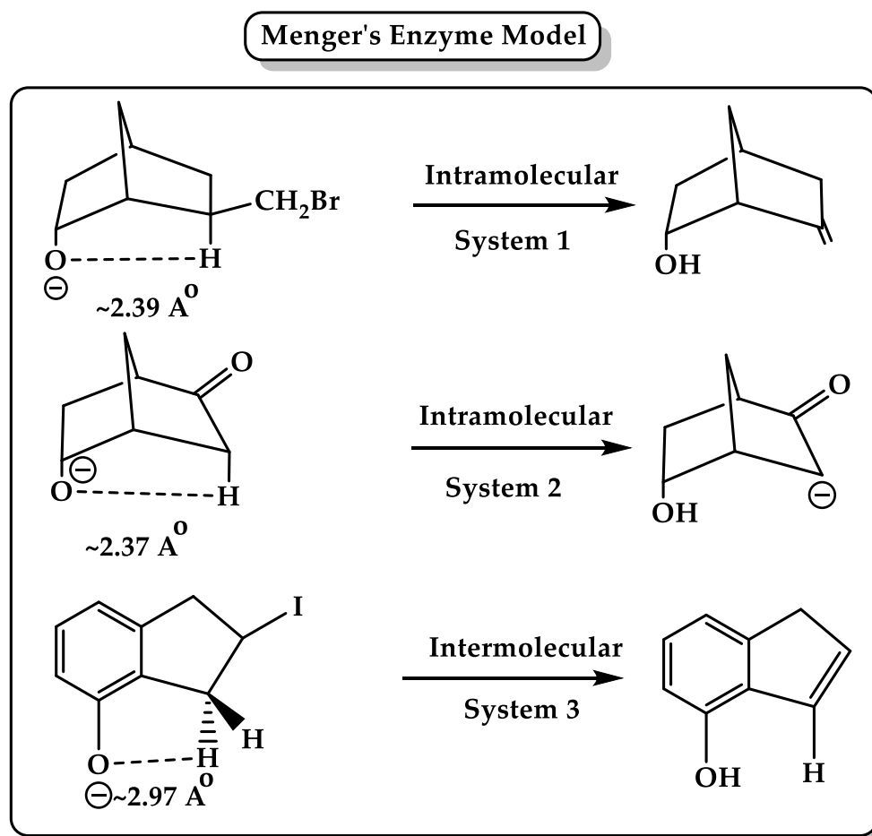
Figure 3. Menger's enzyme model based on "spatiotemporal hypothesis," which suggests that intermolecular or intramolecular reaction is determined by the distance between the two reacting centers of the reactant [66].
