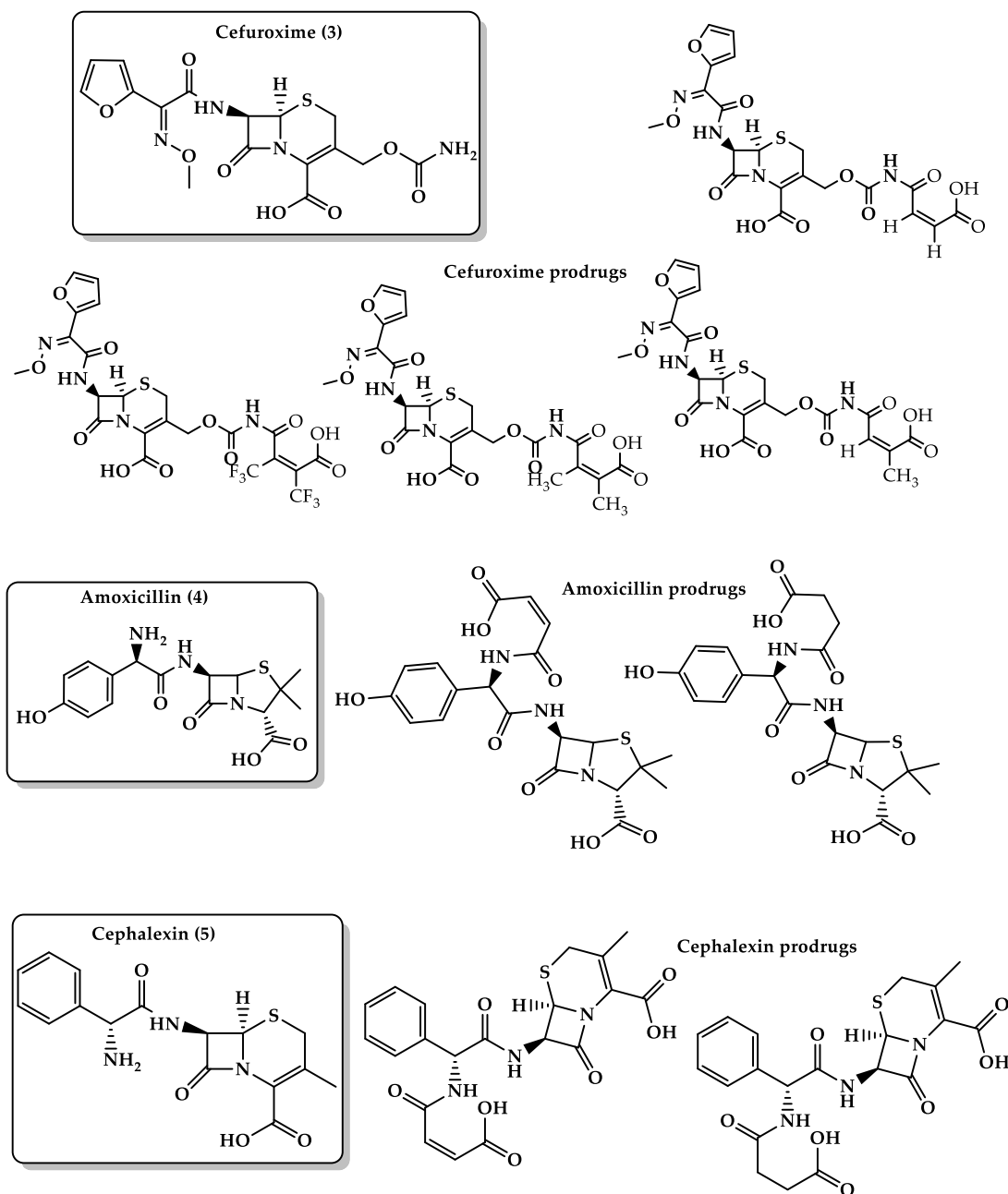
Figure 6. Chemical structures of cefuroxime (3) and cefuroxime prodrugs, amoxicillin (4) and amoxicillin prodrugs, cephalixin (5) and cephalixin prodrugs.
