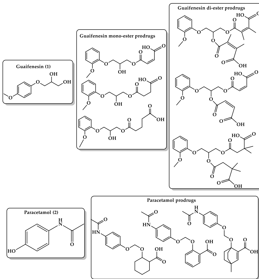
Figure 5. Chemical structures of guaifenesin (1) and guaifenesin prodrugs and paracetamol (2) and paracetamol prodrugs based on Kirby's acetal enzyme model.
