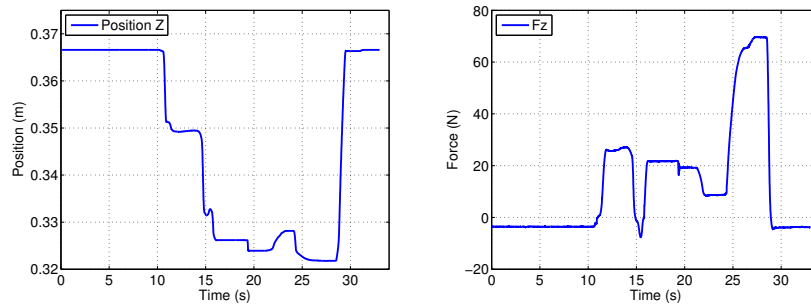
Figure 5.8: The position and force of the end-effector along the Z axis during the positioning task.
