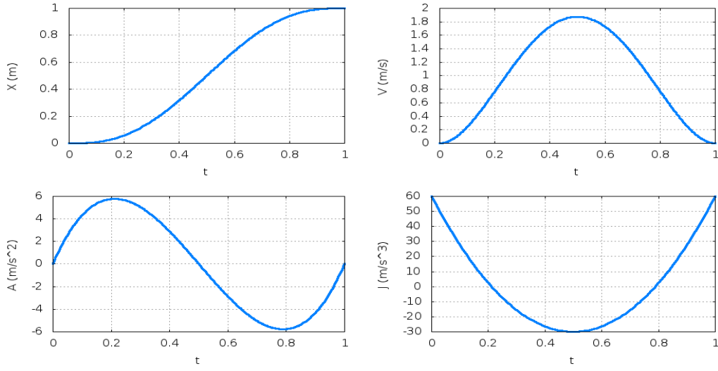
Figure 4.7: One continuous interpolant with 5 th degree polynomial
