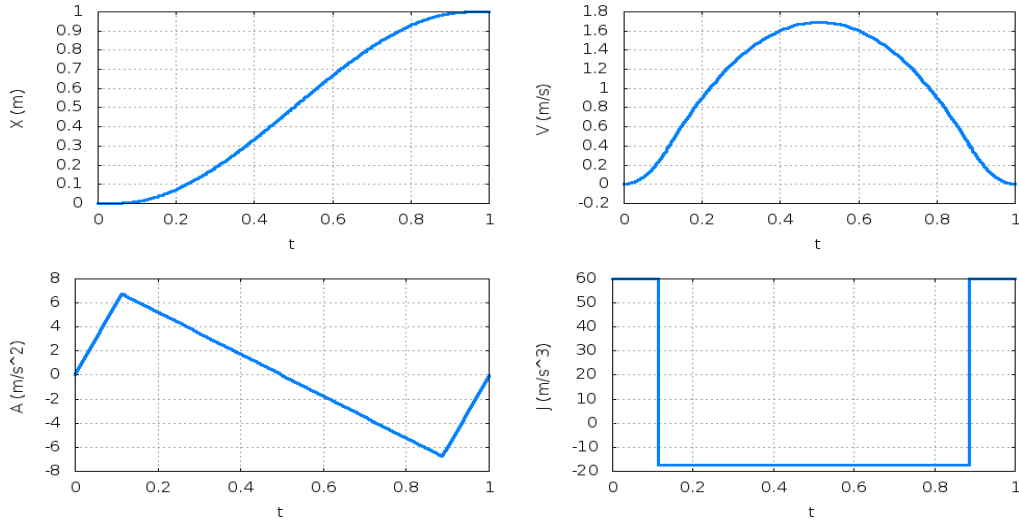
Figure 4.3: 3 rd degree polynomial interpolants with fixed jerk
