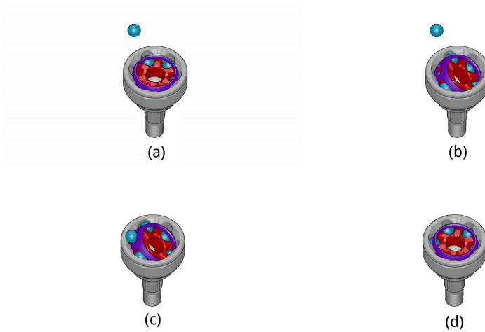
Figure 5.11: Sub-task of the insertion task of one ball. (a): Initial position. (b): Open position. (c): Insertion position. (d): Closed position.
