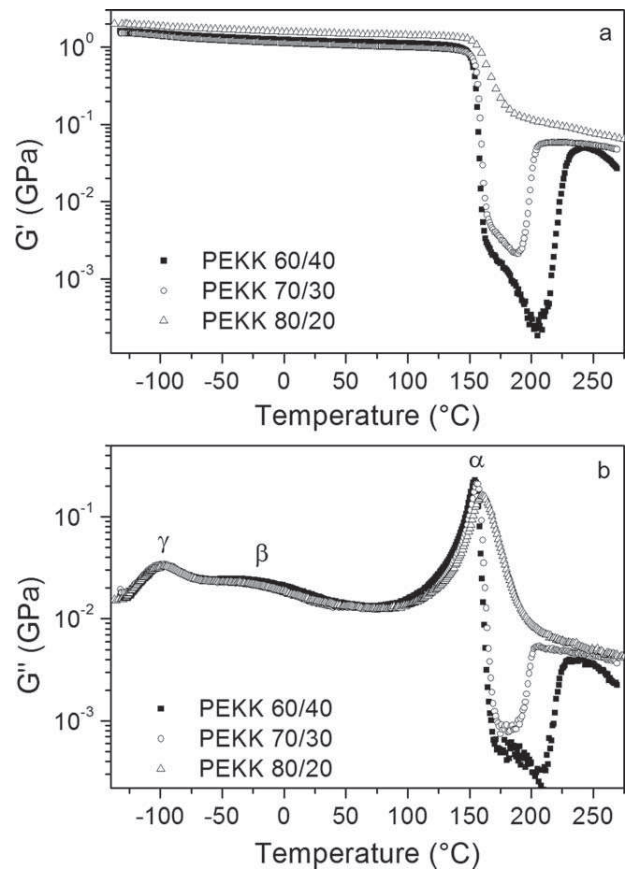
Figure 6. (a) G' versus temperature at 1 rad s -1 for PEKK 60/40, 70/30, and 80/20. (b) G'' versus temperature at 1 rad s -1 for PEKK 60/40, 70/30, and 80/20.
