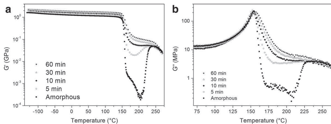
Figure 8. (a) G' versus temperature at 1 \text{ rad s}^{-1} for isothermally crystallized PEKK 60/40 at 245 \text{ }^\circ\text{C} during 5, 10, 30, and 60 min. (b) G'' vs temperature at 1 \text{ rad s}^{-1} for isothermally crystallized PEKK 60/40 at 245 \text{ }^\circ\text{C} during 5, 10, 30, and 60 min.
