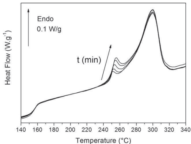
Figure 5. DSC thermograms of isothermally crystallized PEKK 60/40 at 245 °C for 5, 10, 20, 40, and 60 min.
