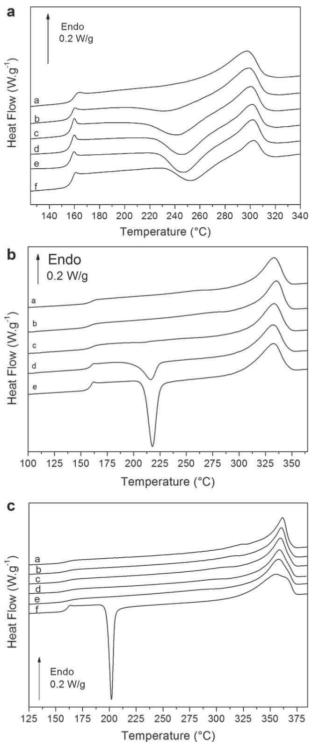
Figure 3. (A) DSC thermograms of PEKK 60/40 at 10\text{ }^{\circ}\text{C min}^{-1} after different cooling rates: (a) 2\text{ }^{\circ}\text{C min}^{-1} , (b) 5\text{ }^{\circ}\text{C min}^{-1} , (c) 10\text{ }^{\circ}\text{C min}^{-1} , (d) 20\text{ }^{\circ}\text{C min}^{-1} , (e) 40\text{ }^{\circ}\text{C min}^{-1} , and (f) quenched. (B) DSC thermograms of PEKK 70/30 at 10\text{ }^{\circ}\text{C min}^{-1} after different cooling rates: (a) 10\text{ }^{\circ}\text{C min}^{-1} , (b) 20\text{ }^{\circ}\text{C min}^{-1} , (c) 40\text{ }^{\circ}\text{C min}^{-1} , (d) 60\text{ }^{\circ}\text{C min}^{-1} , and (e) quenched. (C) DSC thermograms of PEKK 80/20 at 10\text{ }^{\circ}\text{C min}^{-1} after different cooling rates: (a) 5\text{ }^{\circ}\text{C min}^{-1} , (b) 10\text{ }^{\circ}\text{C min}^{-1} , (c) 20\text{ }^{\circ}\text{C min}^{-1} , (d) 40\text{ }^{\circ}\text{C min}^{-1} , (e) 60\text{ }^{\circ}\text{C min}^{-1} , and (f) quenched.
