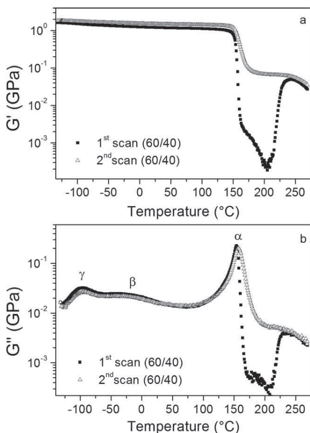
Figure 7. (a) G' versus temperature at 1 \text{ rad s}^{-1} for PEKK 60/40 at first and second scan. (b) G'' versus temperature at 1 \text{ rad s}^{-1} for PEKK 60/40 at first and second thermogram.
