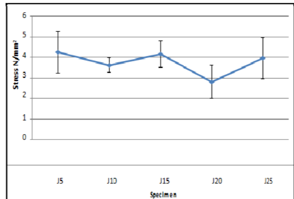
Figure 10 : Tensile strength for all specimens
