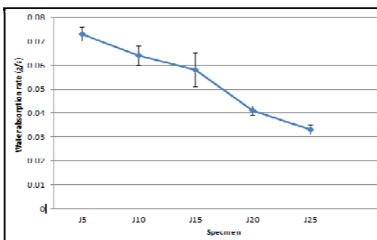
Figure 13 : Water absorption results for all specimens
