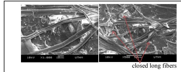
Figure 14 : Surface texture magnification using FESEM
