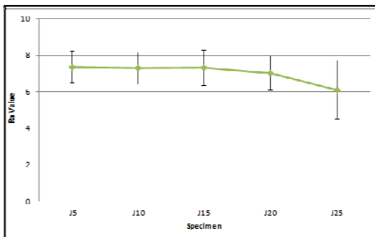
Figure 12 : Surface roughness result
