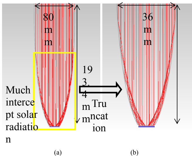
Fig. 3 Ray trace diagram at normal incidence angle ( 0^\circ ) (a) Initial CPC design (b) Truncated CPC design
