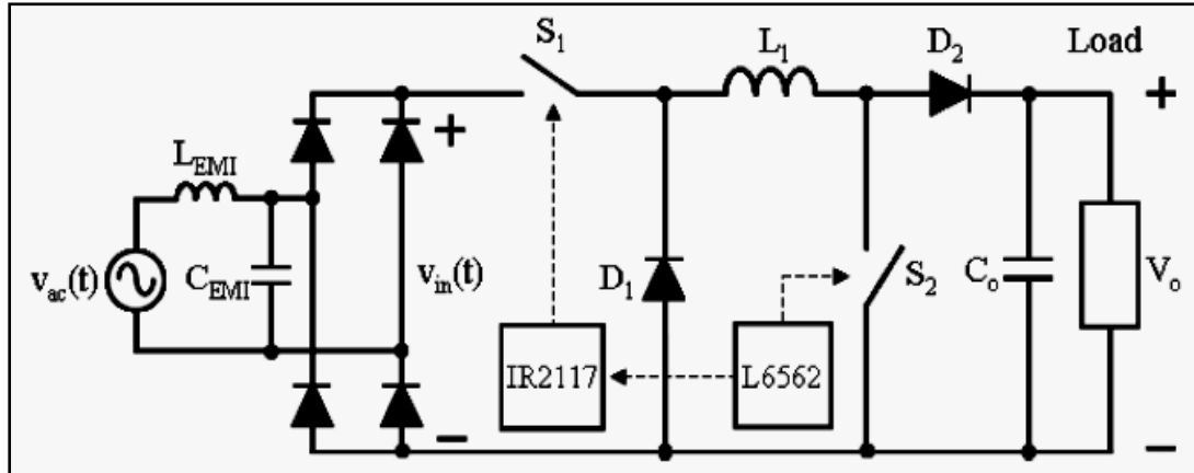
Figure 2.7: Prototype Circuit for the Proposed BCM Non-Inverting Buck Boost PFC Converter
