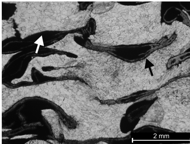
Fig. 6. Polished cross section of a compressed MMSF (AlCu5-GM-O)
