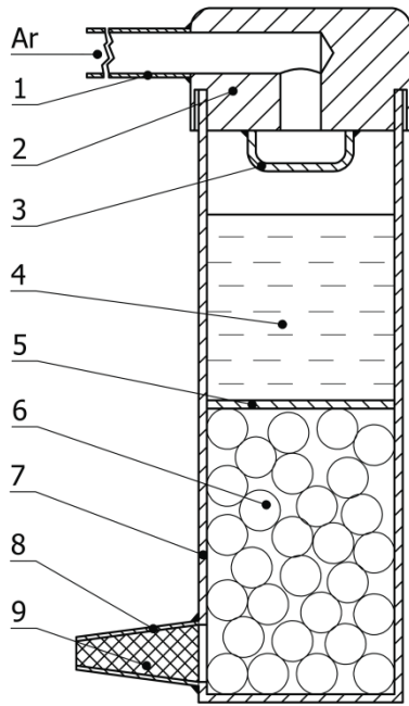
Fig. 2. Schematic sketch of the infiltration system
