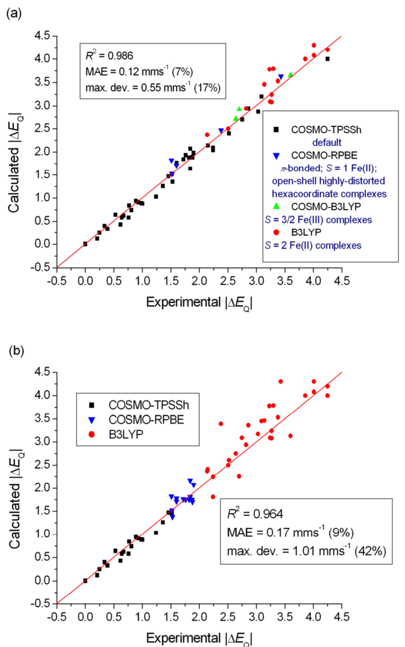
Figure 5. Comparison of experimental and DFT-calculated quadrupole splittings ( \Delta E_Q ), applying exchange-correlation functionals for different (a) chemical classes of Fe complexes and (b) ranges of experimental \Delta E_Q (in combination with the STO-TZP basis set). The red line was drawn at \Delta E_Q(\text{exp.}) = \Delta E_Q(\text{calc.})
