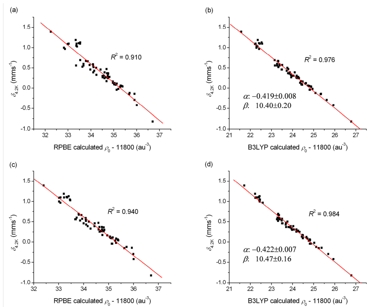
Figure 2. Linear correlations between the (a) RPBE, (b) B3LYP, (c) COSMO-RPBE, (d) COSMO-B3LYP (in combination with the STO-CP(PPP) basis set) calculated electron density ( \rho_0 ) at the ^{57}\text{Fe} nucleus and the corrected experimental isomer shift ( \delta_{4,2K} ). The fitting parameters are indicated for the B3LYP method, for all other applied DFT methods the results are shown in the SI.
