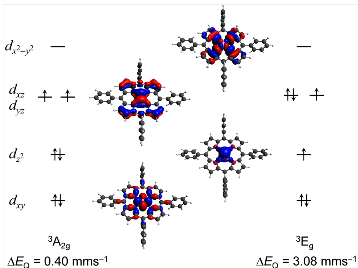
Figure 6. Schematic representation of the electronic configurations and the 3D illustration of the DFT Fe-3d orbitals of the triplet {}^3A_{2g} and {}^3E_g ( D_{4h} ) states of Fe(TPP) ( 35 ). Note that for the sake of simplicity we do not show spin-polarized energy levels and we only show one component of the degenerate d_{xz} , d_{yz} orbitals and {}^3E_g states. The given \Delta E_Q values were computed at the B3LYP / STO-TZP level of theory and are to be compared with the experimental value of 1.51 \text{ mms}^{-1} .
