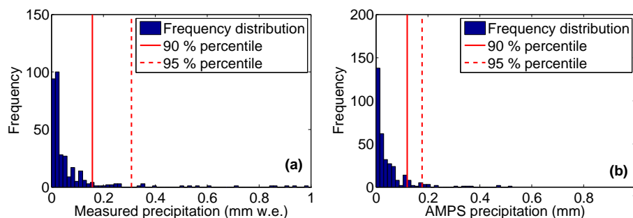
Figure 3. (a) Histogram of the precipitation measurements in mm w.e. with a distance of 0.015 mm w.e. between the bins; the two highest values (1.4 and 2.1 mm w.e.) are not shown. (b) Histogram of the precipitation simulations from AMPS with the same distance of 0.015 mm between the bins.
