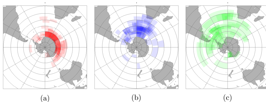
Figure 12. Estimated source regions of the modelled and measured precipitation events for the available trajectories arriving at (a) 600 hPa, (b) 500 hPa, and (c) 300 hPa. The stronger the colour, the more frequently the respective source area was found.
