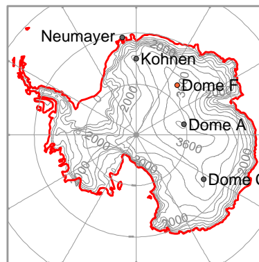
Figure 1. AMPS topography of Antarctica and location of selected stations.
