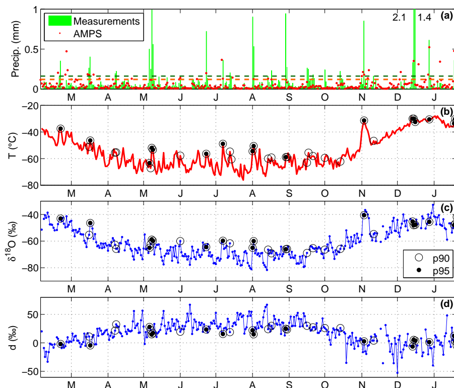
Figure 2. (a) Measurements and AMPS simulations of daily precipitation in mm w.e. Green dashed line: 90 % percentiles from measurements. Orange dashed line: 90 % percentile from AMPS. (b) Daily measurements of temperature, (c) daily measurements of \delta^{18}\text{O} , and (d) daily measurements of deuterium excess. The open and filled circles in panels (b–d) mark the days where the precipitation exceeded the 90 and 95 % percentiles respectively. The 90 % percentile is defined as the threshold for precipitation events.
