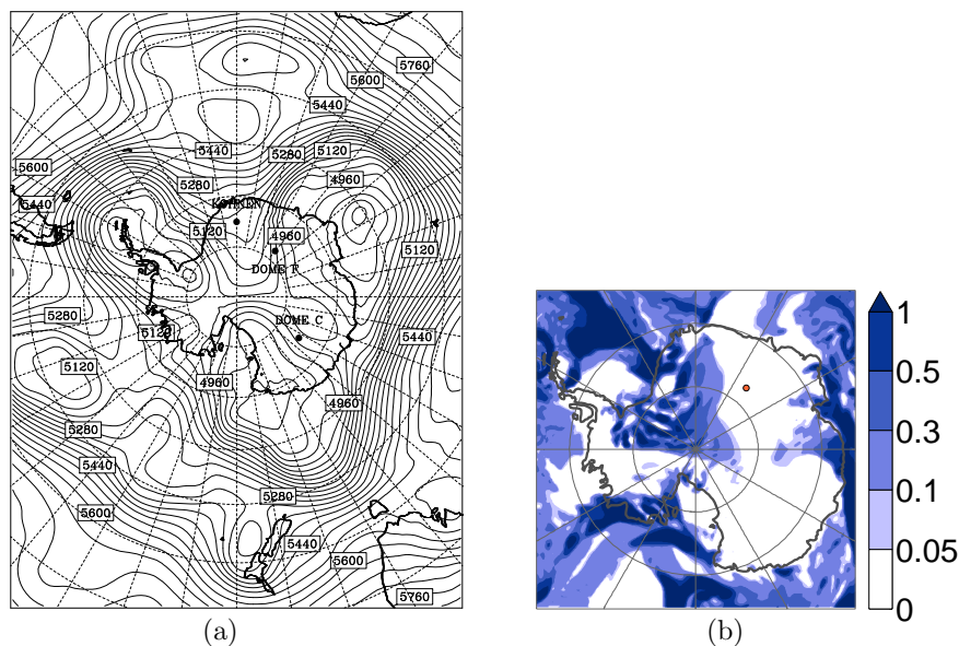
Figure 8. Example for the event Southerly Flow; (a) 500 hPa geopotential height from AMPS, 1 October 2003 00:00 UTC, (b) 6 h precipitation in mm from AMPS, 1 October 2003 00:00 UTC.
