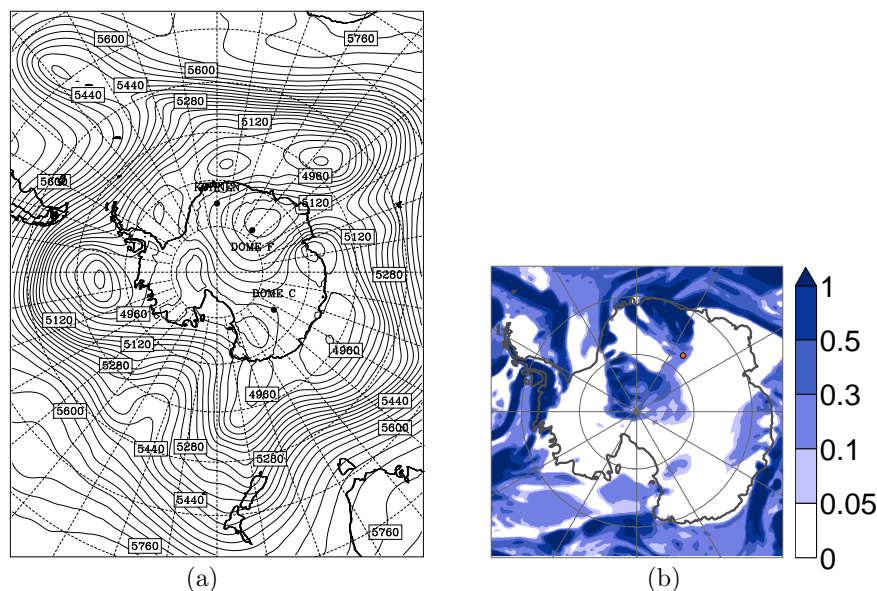
Figure 7. Example of a blocking high: (a) 500 hPa geopotential height from AMPS, 3 November 2003 00:00 UTC, (b) 6 h precipitation in mm from AMPS, 3 November 2003 00:00 UTC.
