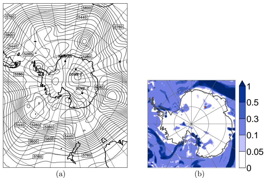
Figure 9. Example for the event type Previous Precipitation Event; (a) 500 hPa geopotential height from AMPS, 14 December 2003 00:00 UTC, (b) 6 h precipitation in mm from AMPS, 14 December 2003 00:00 UTC.
