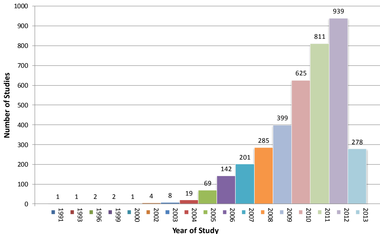
Figure 7.2. The number of studies addressing the toxicity of a nanomaterial to humans, organized by year of publication, as of September 2013. Approximately 1800 of these studies can be found in the searchable database being developed by OSHA. (Figure courtesy of J. Carter.)
