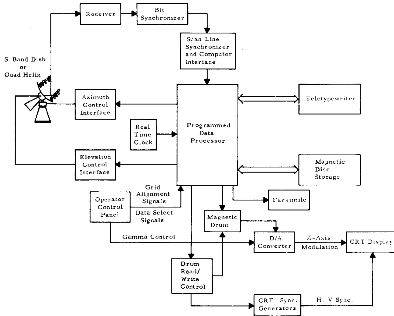
Figure 5-2 Block Diagram of APT Receiver Station.
