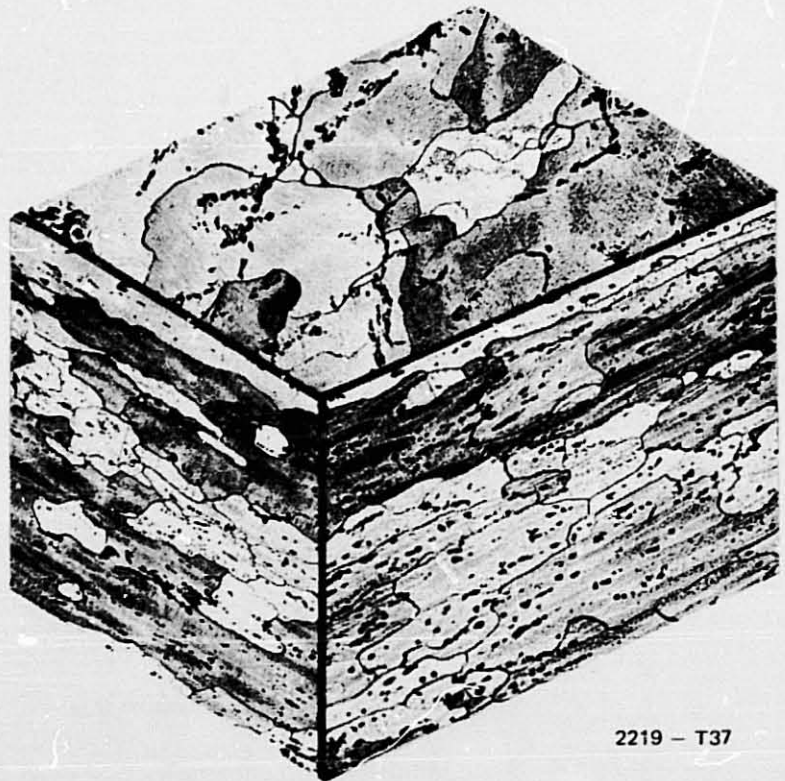
FIG. 1 GRAIN STRUCTURE AT MIDPLANE OF PLATE OF 7075 (2.500") AND 2219 (2.00") ALLOYS
