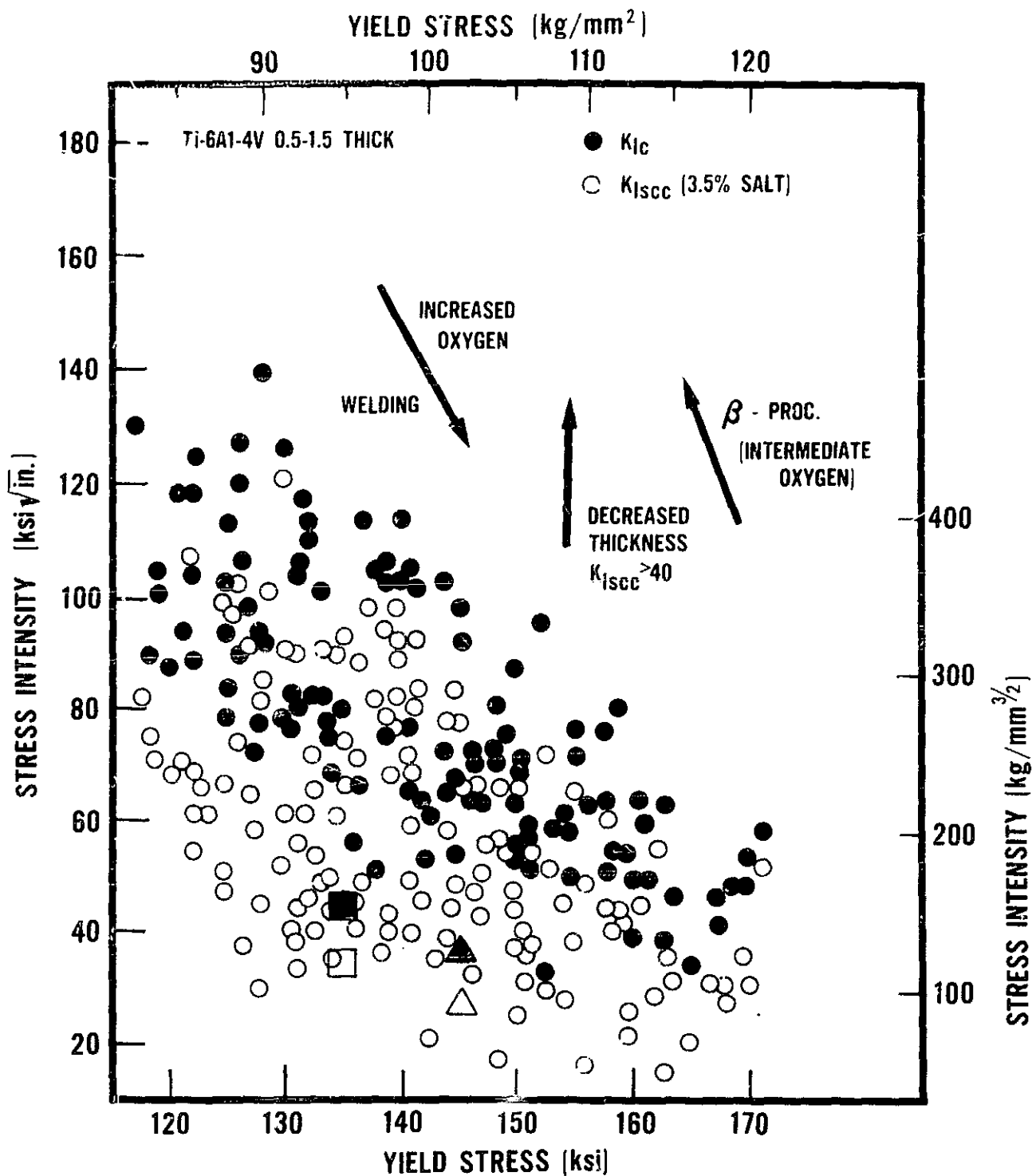
FIG.103 THE VARIATION OF K_{Ic} AND K_{IscC} WITH YIELD STRENGTH FOR THE ALLOY Ti-6Al-4V. (REF. 42)
