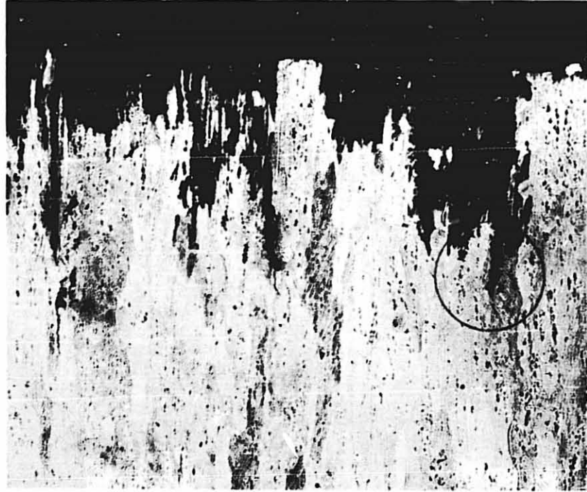
FIG. 18a DEEP DIRECTIONAL PITTING IN S.T. TENSION SPECIMEN OF 2219 - T87 (338148 - N8) THAT FAILED AFTER 42 DAYS EXPOSURE TO 3.5% NaCl - A.I. AT A STRESS OF 75% Y.S. KELLER'S ETCH (100X)
