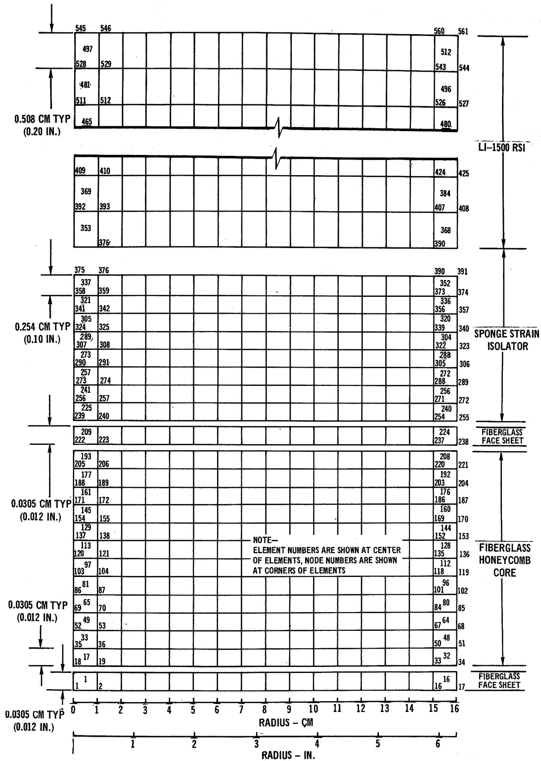
COMPUTER MODEL - SINGLE-LAYER RSI ANTENNA WINDOW DESIGN FOR C-BAND ANTENNA SYSTEM
