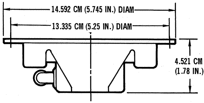
C-Band Horn Antenna
