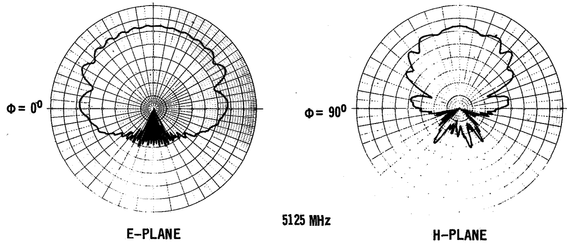
C-BAND SLOT PATTERNS WITH SIMULATED RSI - 5.08 CM (2.0 IN.) THICK
