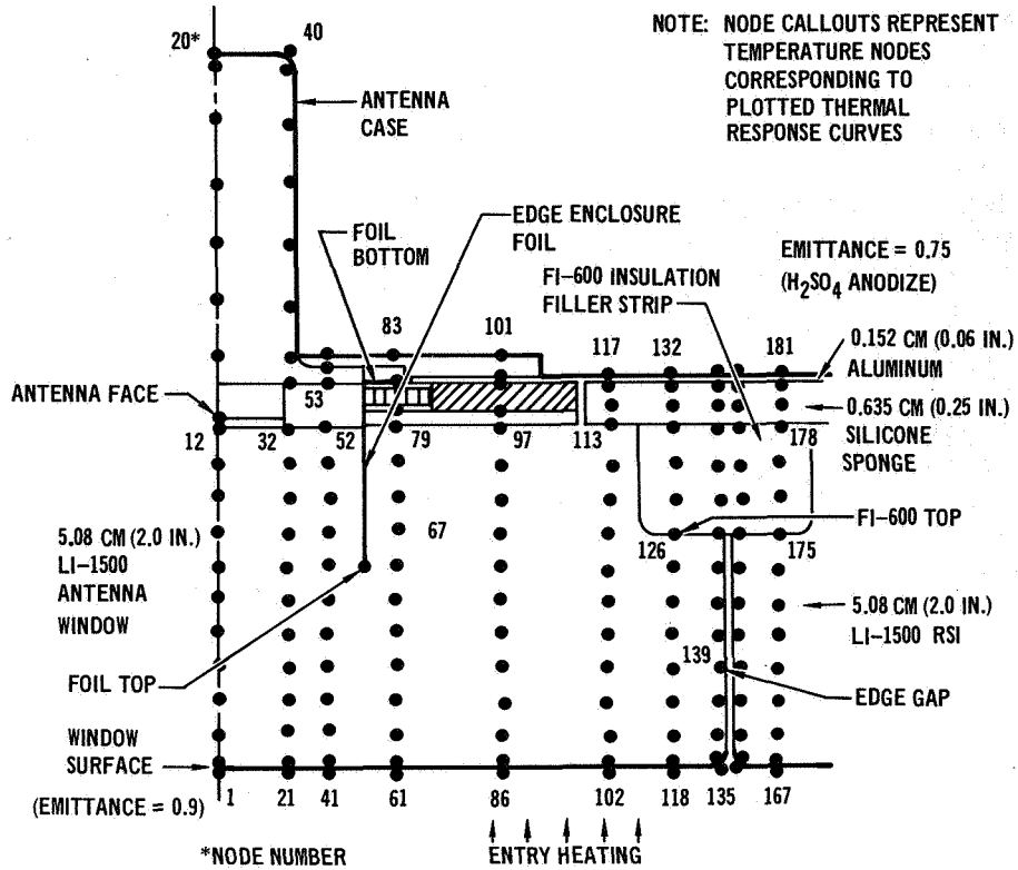
C-BAND SLOT ANTENNA SYSTEM THERMAL MODEL
