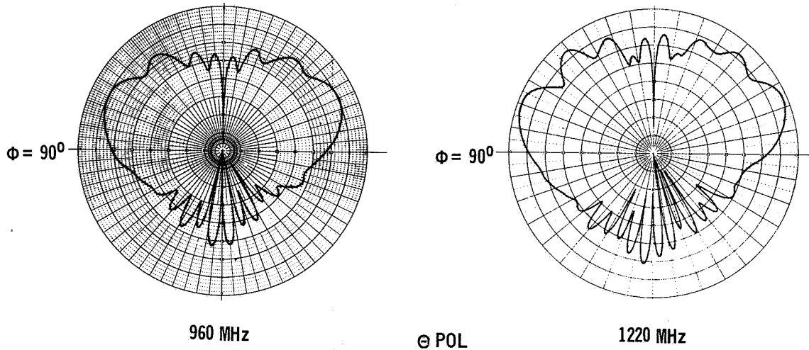
L-BAND PATTERNS WITH SIMULATED RSI RADIAL-1.83M (6 FT) DIAMETER GROUND PLANE
