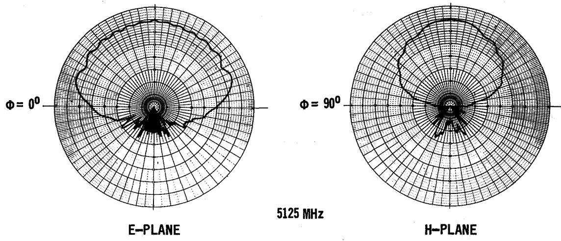
C-BAND SLOT REFERENCE PATTERNS - 76.2 x 76.2 CM (30.0 x 30.0 IN.) GROUND PLANE
