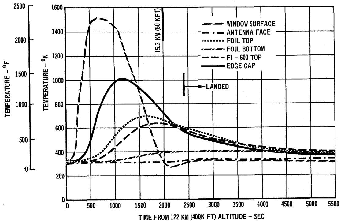
C-BAND SLOT ANTENNA SYSTEM ENTRY THERMAL RESPONSE
