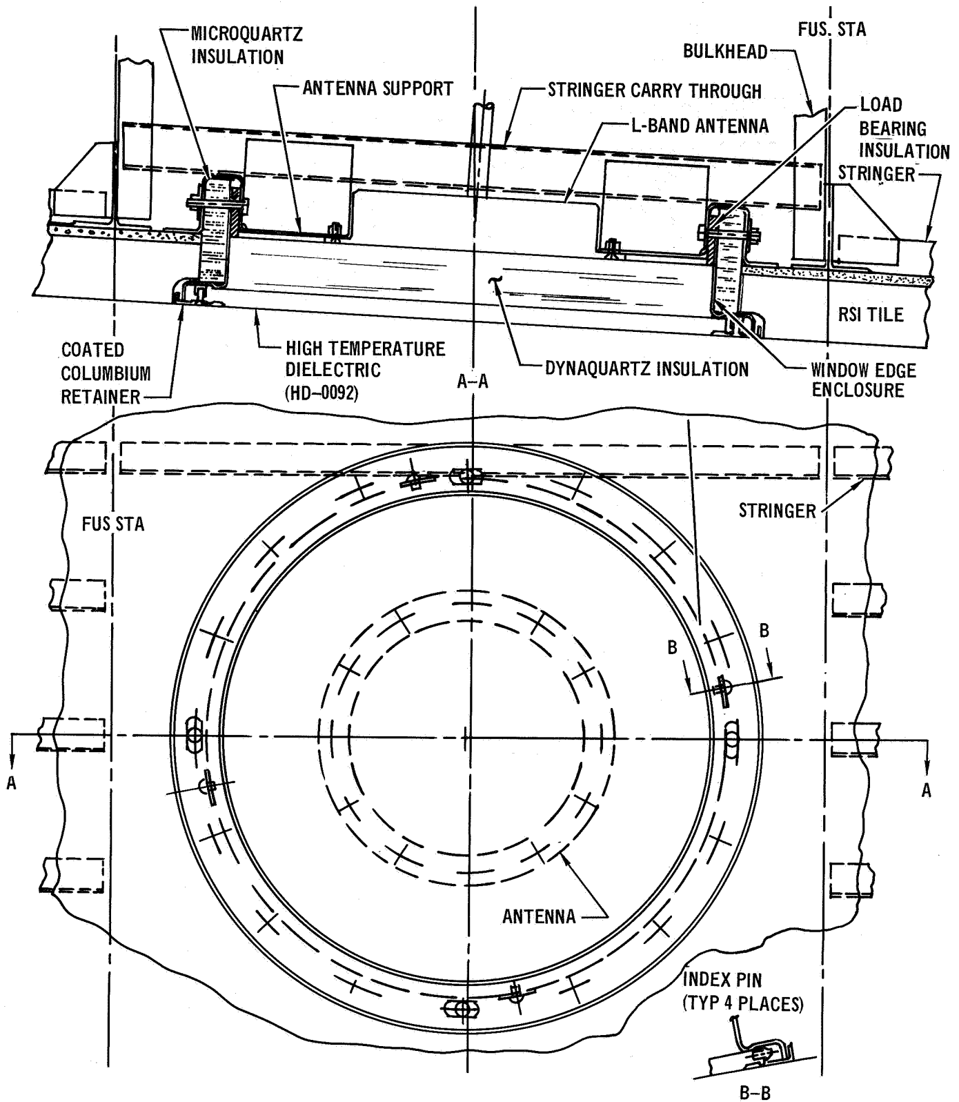
MULTIPLE-LAYER ANTENNA WINDOW DESIGN – MAXIMUM WINDOW SIZE
