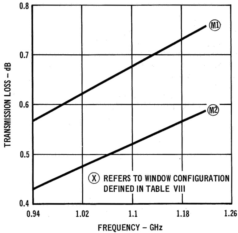
TRANSMISSION LOSS THRU MULTIPLE-LAYER ANTENNA WINDOWS AT L-BAND
