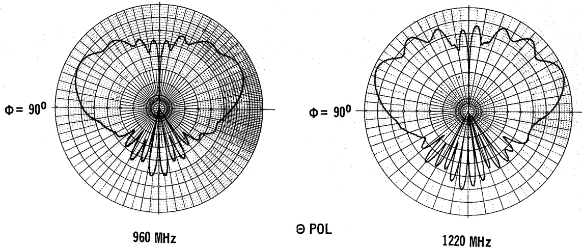
L-BAND PATTERNS WITH SIMULATED RSI-1.83M (6 FT) DIAMETER GROUND PLANE
