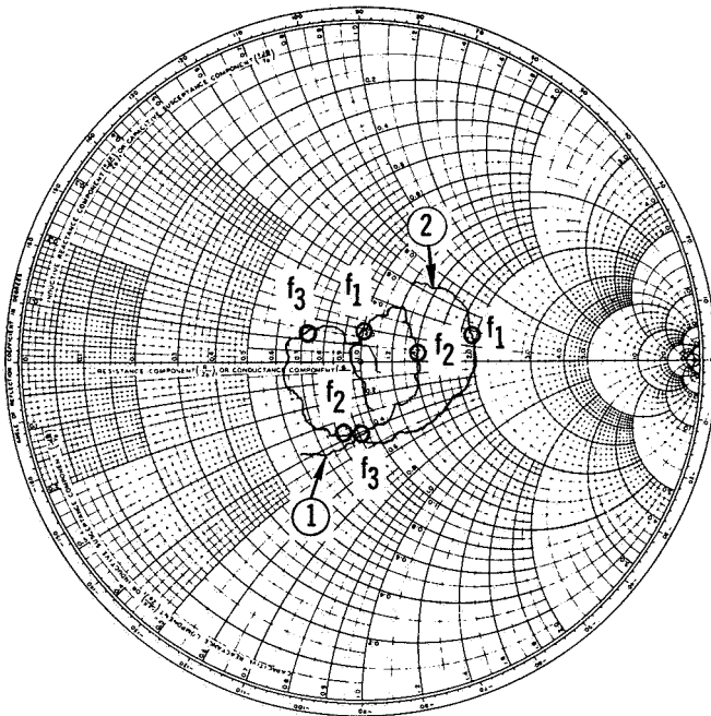
L-BAND IMPEDANCE – 31.75 CM (12.5 IN.) DIAMETER WINDOW
