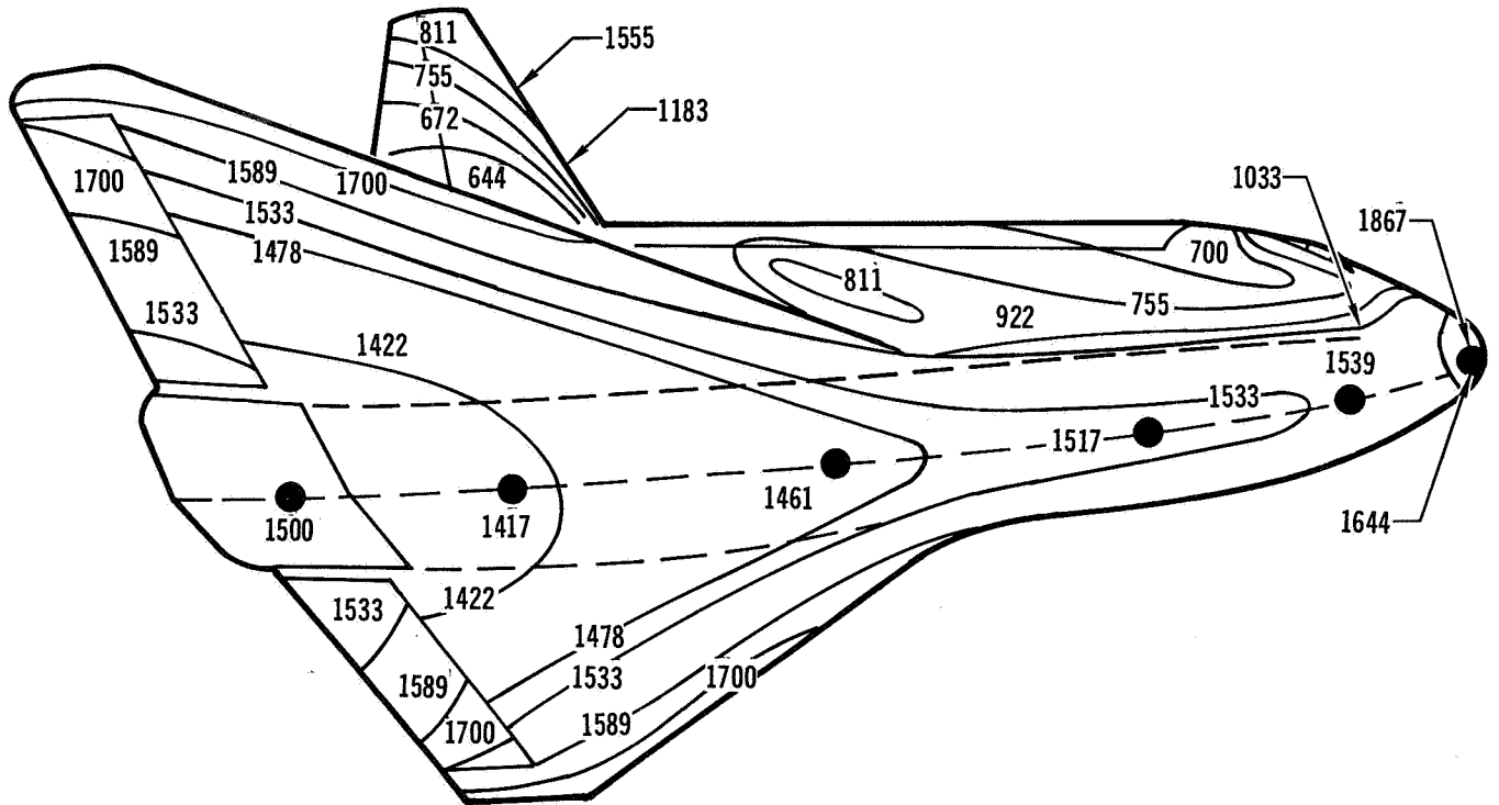
ENTRY TEMPERATURES °K
