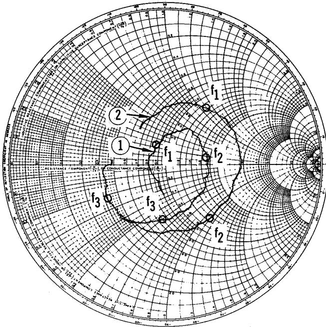
L-BAND IMPEDANCE – 27.94 CM (11.0 IN.) DIAMETER WINDOW
