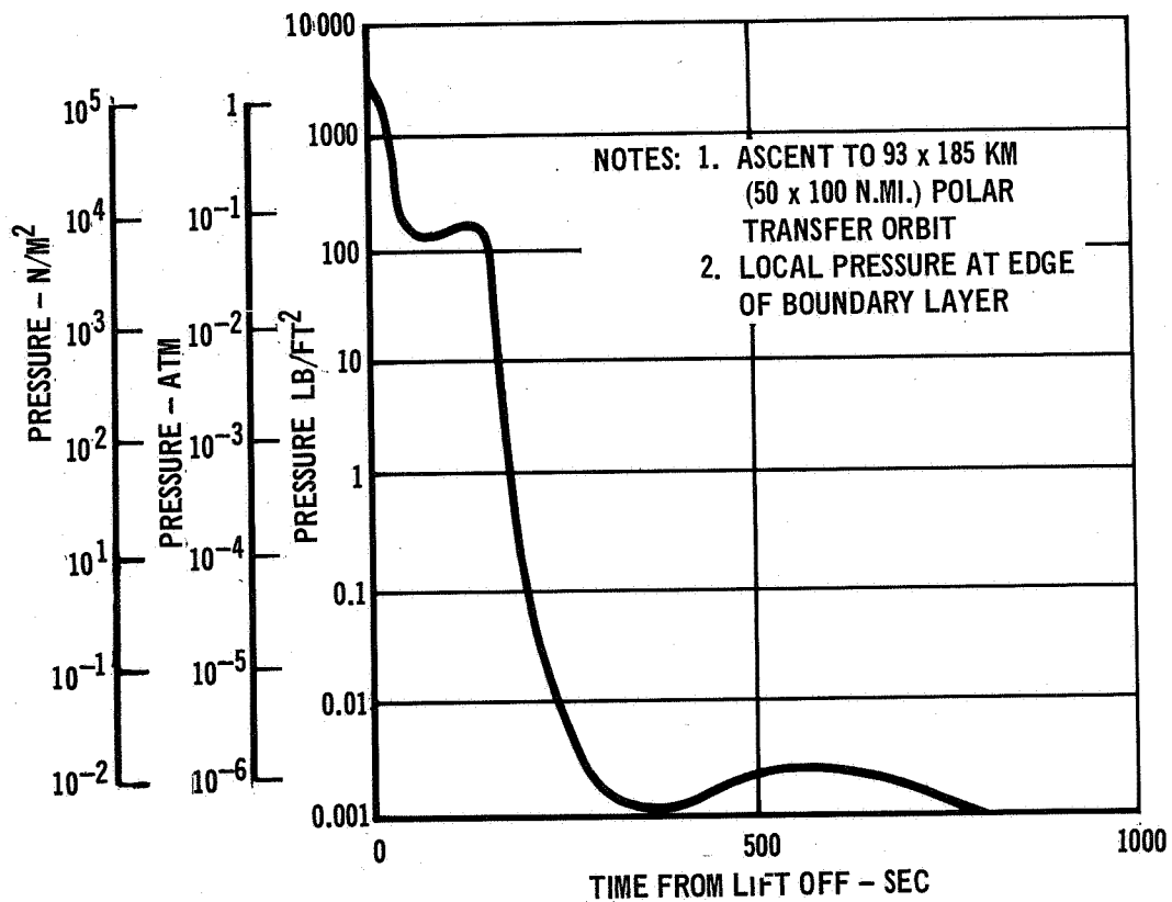
ASCENT LOCAL STATIC PRESSURE HISTORY
