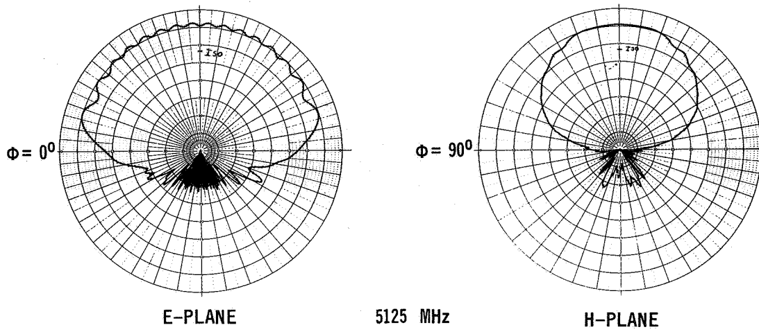
C-BAND SLOT REFERENCE PATTERNS
