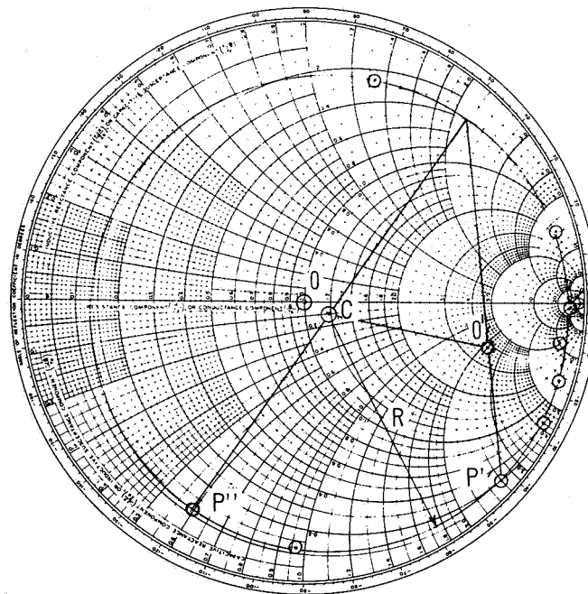
f = 960 MHz
