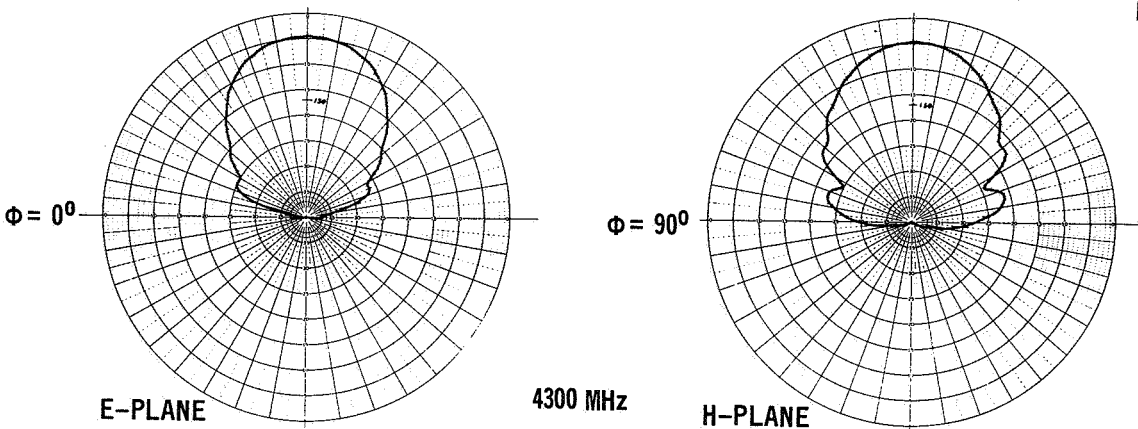
C-BAND HORN PATTERNS – 15.24 CM (6.0 IN.) DIAMETER WINDOW AND 5.08 CM (2.0 IN.) SIMULATED RSI
