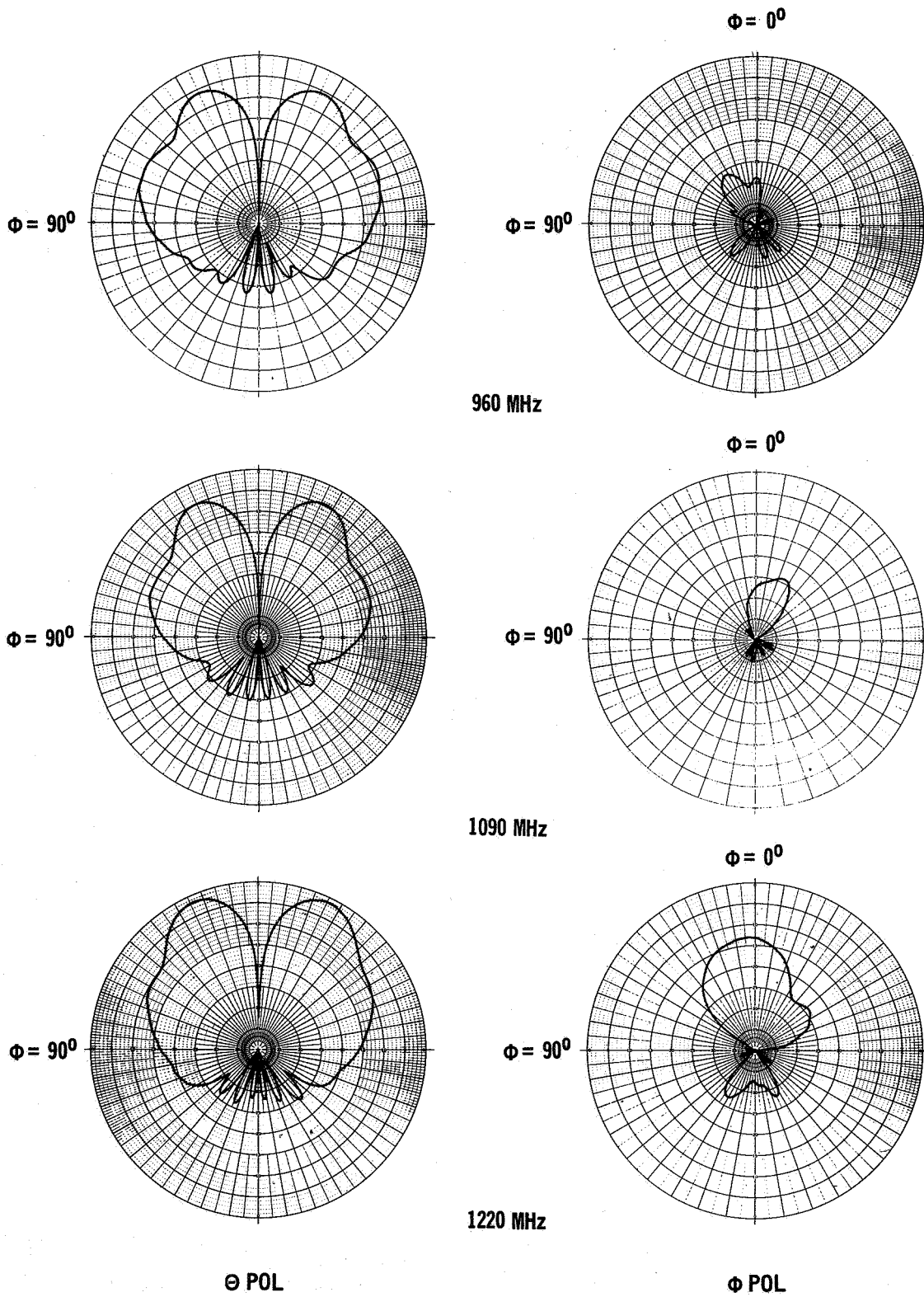
L-BAND PATTERNS – MULTIPLE-LAYER WINDOW AND SIMULATED TPS
