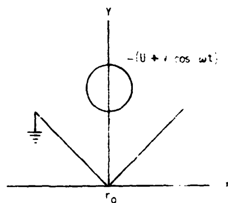
Figure 7b. Monopole electrodes (end view).
