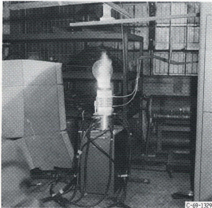
Figure 12. - Radiofrequency plasma torch operating at 500-kilowatt plate power with air.
