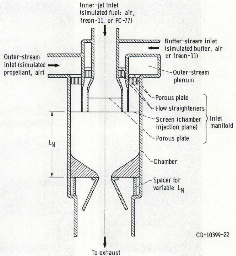
(b) Schematic of coaxial-flow test apparatus at UARL.
