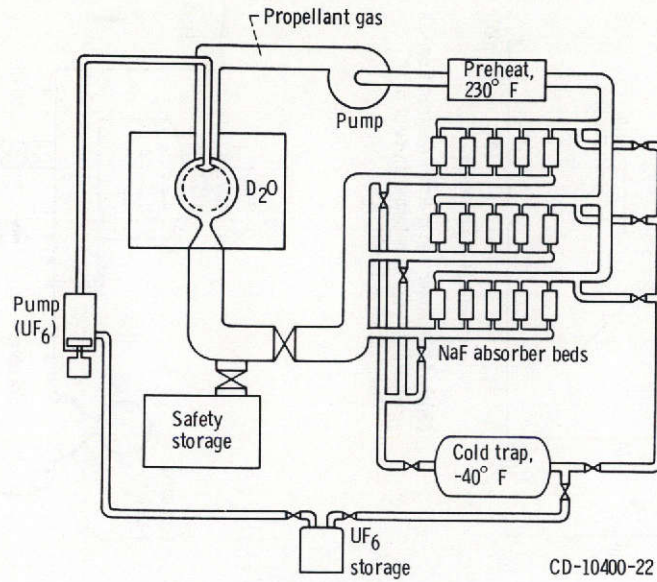
Figure 11. - Cold-flow critical experiment.
