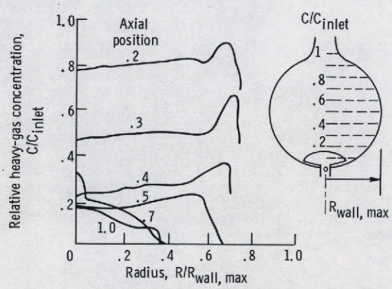
Figure 4. - Heavy-gas distribution in curved porous-wall apparatus at mass flow ratio of 100 to 1.
