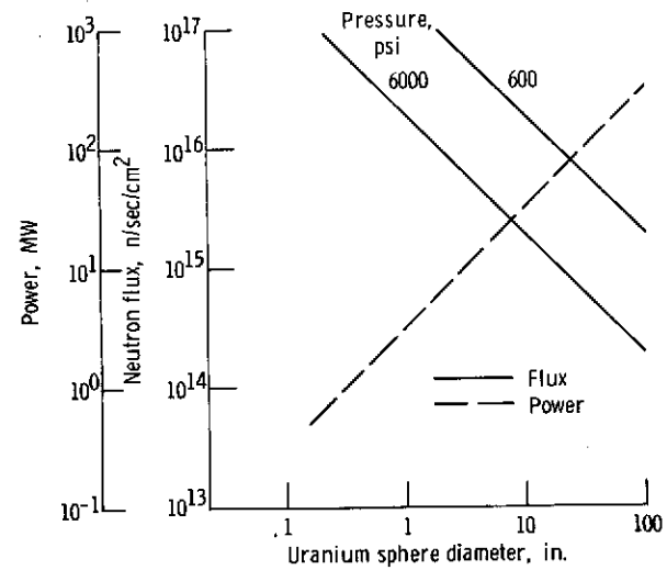
Figure 14. - Power and thermal neutron flux required to keep edge temperature of uranium plasma at 11 000° R.
