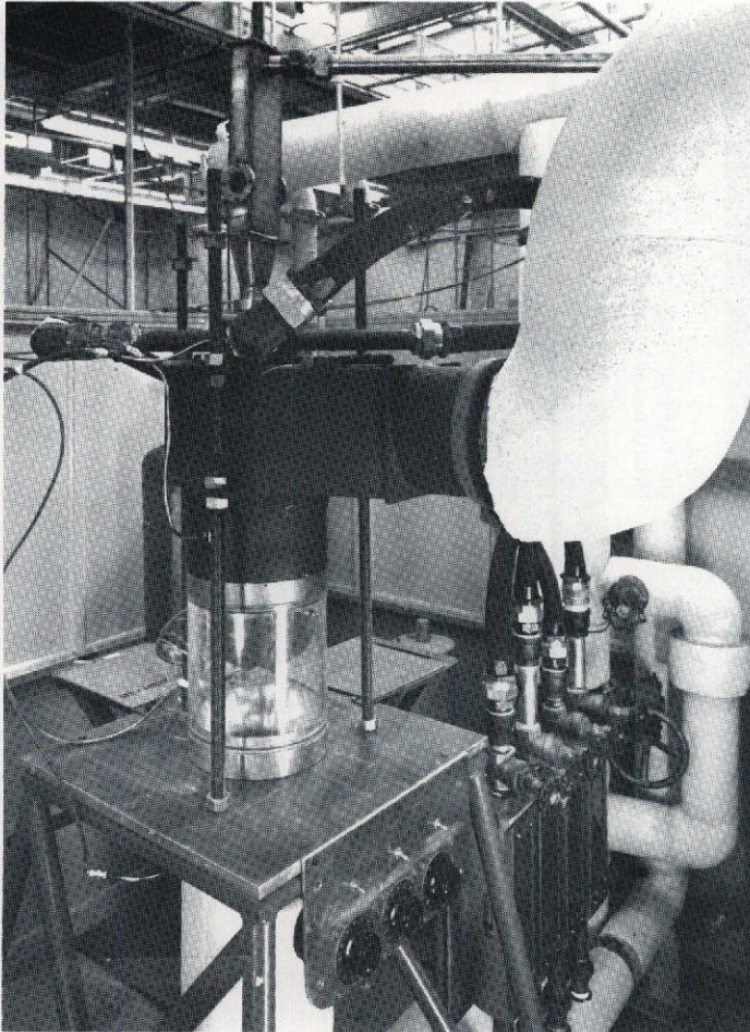
(a) Photograph of coaxial-flow test apparatus at UARL.
