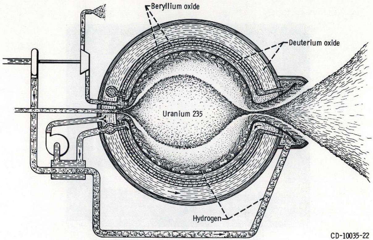
Figure 1. - Lewis gas core nuclear rocket concept.
