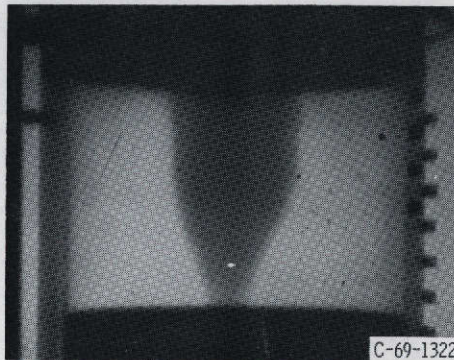
(e) Outer- to inner-mass-flow ratio of 130 showing good fuel-region containment; thick porous material across inlet face.
