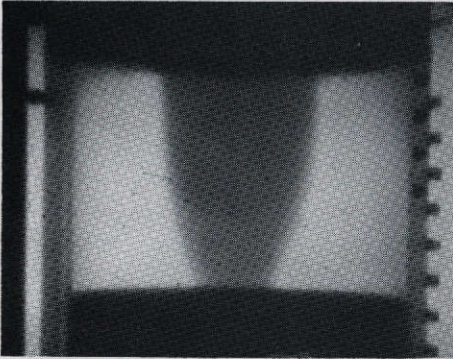
(c) Outer- to inner-mass-flow ratio of 30 showing good fuel-region containment; thick porous material across inlet face.
