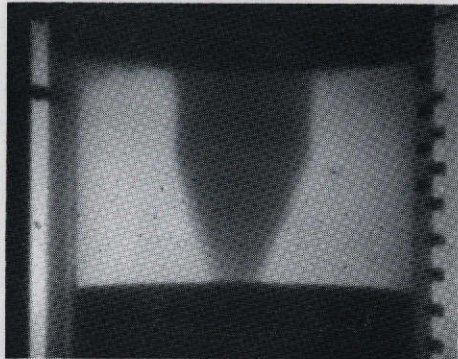
(d) Outer- to inner-mass-flow ratio of 80 showing good fuel-region containment; thick porous material across inlet face.
