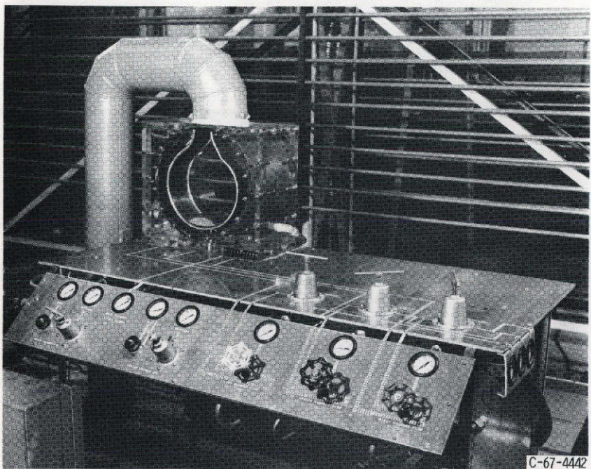
Figure 2. - Two-dimensional experiment mockup of Lewis gas core concept.
