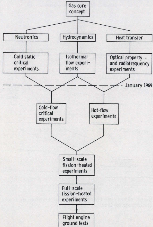
Figure 10. - Steps required to demonstrate gas core reactor feasibility.
