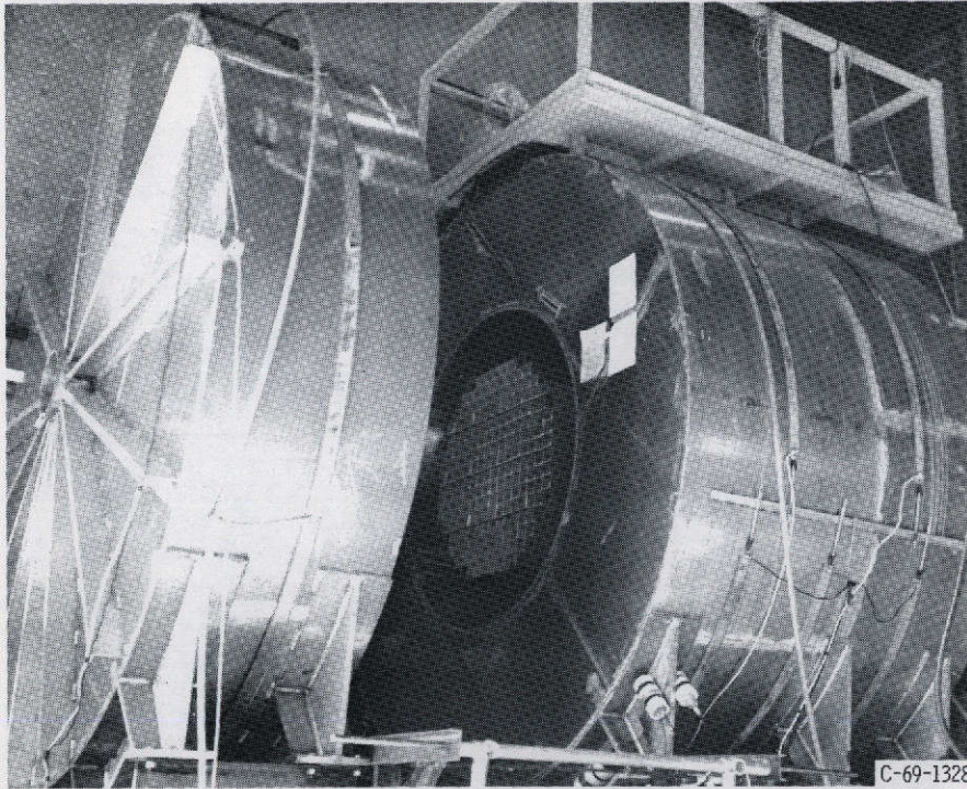
Figure 9. - Full-scale gas core critical experiment facility.
