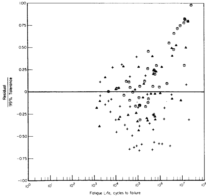
b. Distribution of weighted residuals. Figure D4. - 2024-T4 Bar and rod (notched).
